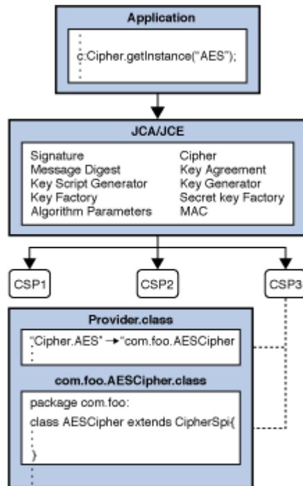
Figure 3-1 Engine Classes
