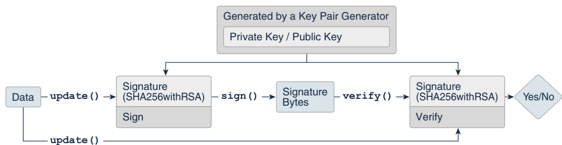
Figure 2-7 Signature Class
