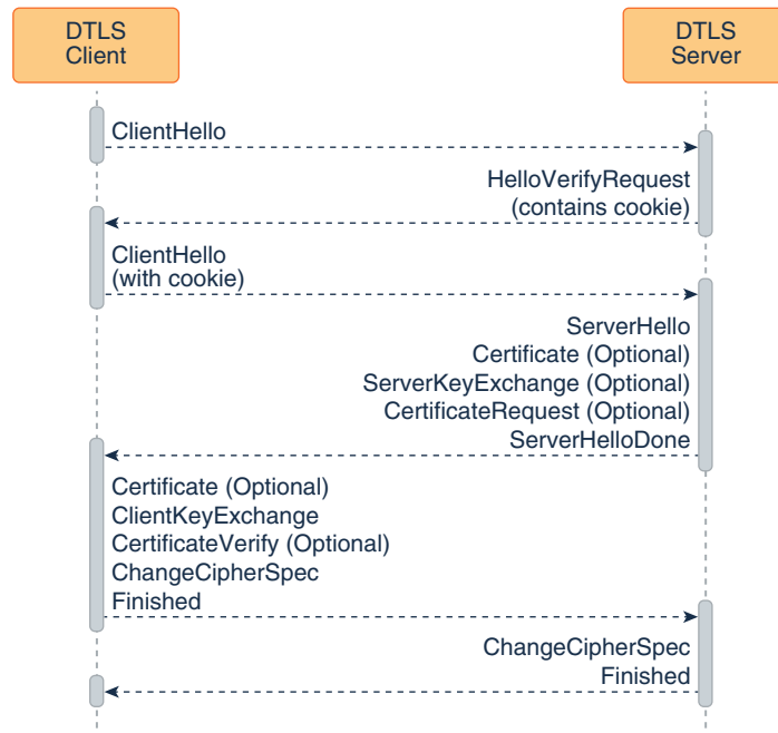
Figure 8-11 DTLS Handshake
