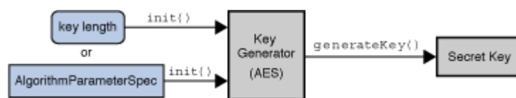
Figure 2-14 The KeyGenerator Class
