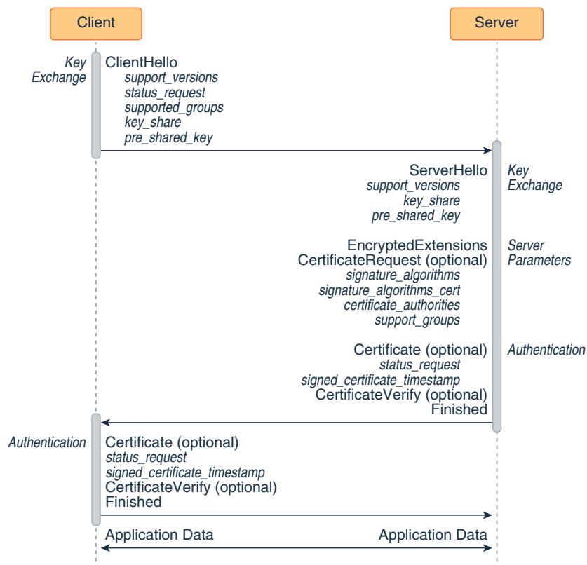
Figure 8-7 TLS 1.3 Handshake
