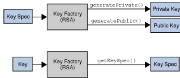
Figure 2-11 KeyFactory Class
