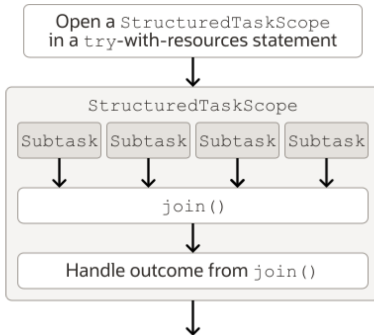
Figure 14-2 Using the StructuredTaskScope Interface
