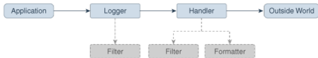
Figure 8-1 Java Logging Control Flow
