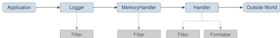
Figure 8-2 Java Logging Control Flow with MemoryHandler
