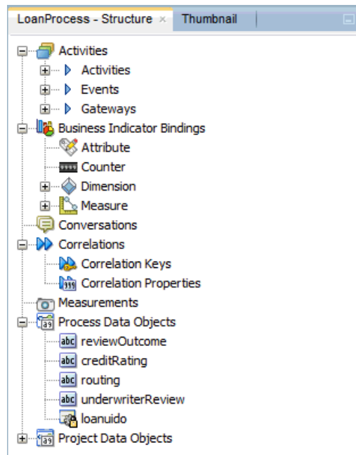
Figure 1-7 Structure View
