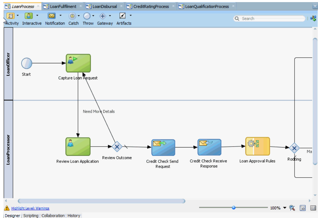
Figure 1-4 Process Editor
