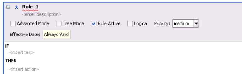
Figure 32-37 Advanced Settings
