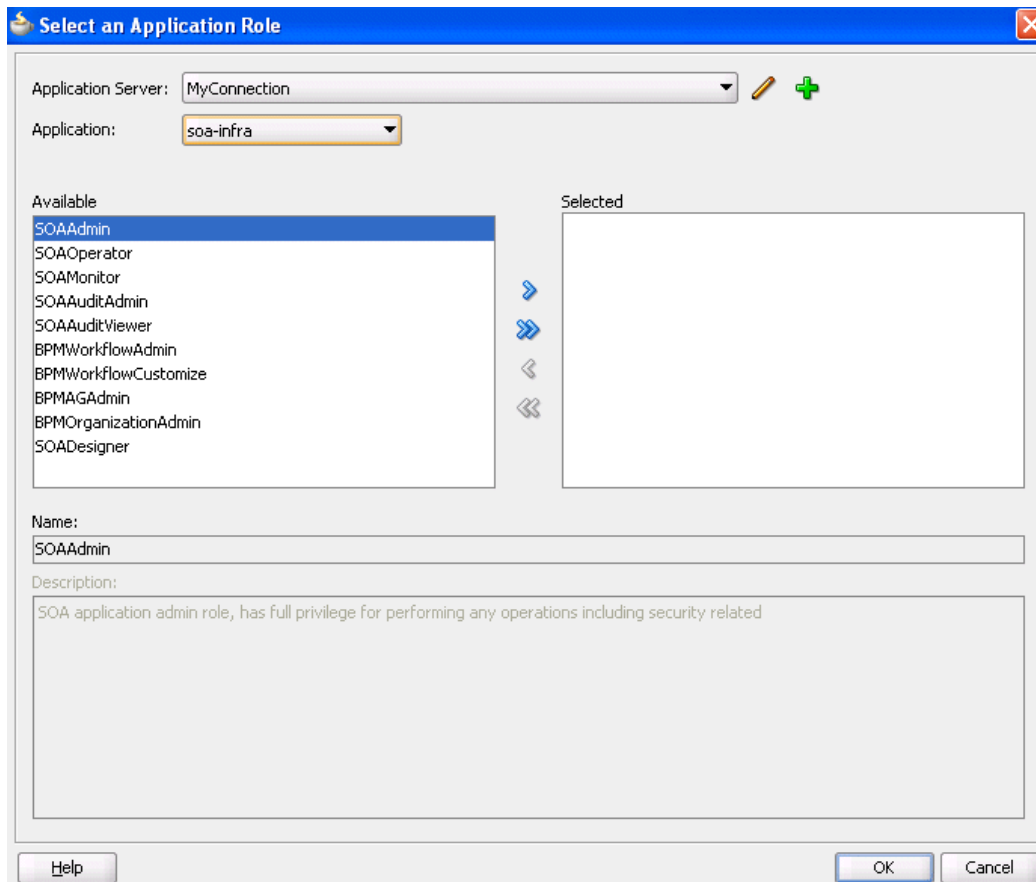
Figure 29-10 Application Role
