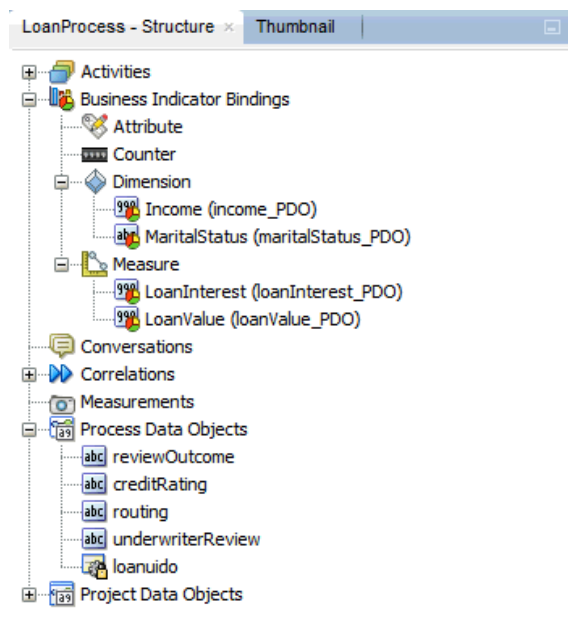
Figure 5-1 Structure Window
