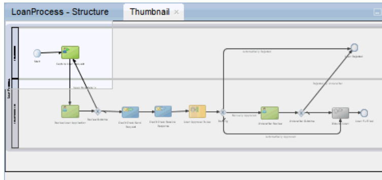
Figure 1-8 Thumbnail View
