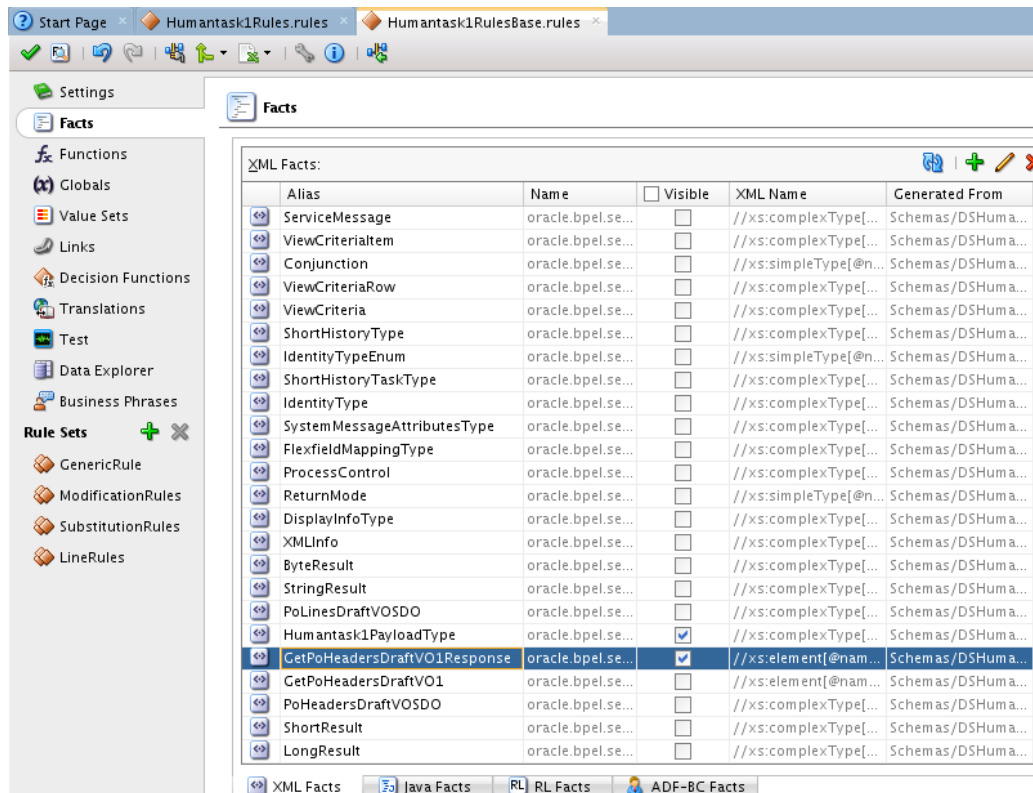
Figure 32-34 Facts List
