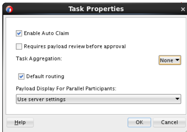
Figure 32-40 Task Properties
