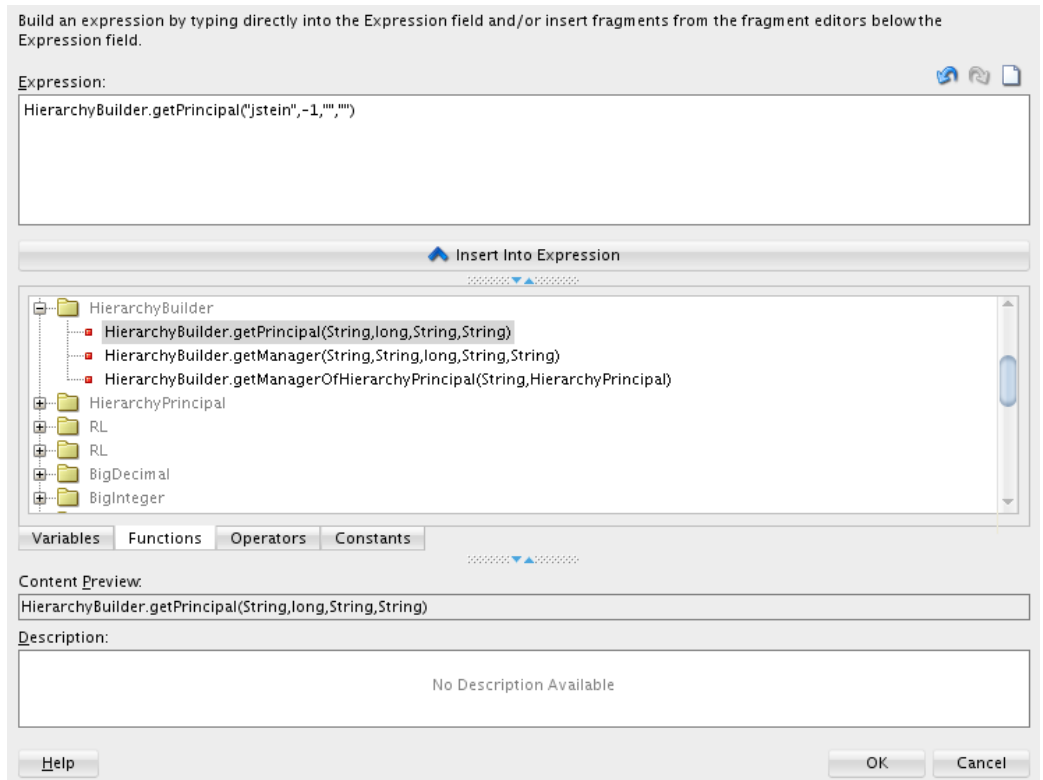
Figure 32-28 HierarchyBuilder Function
