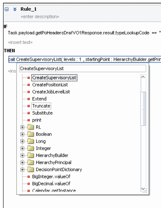
Figure 32-32 Rule Functions
