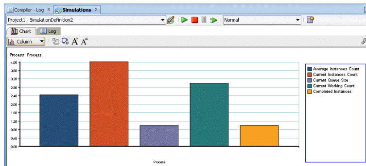
Figure 1-9 Simulation View
