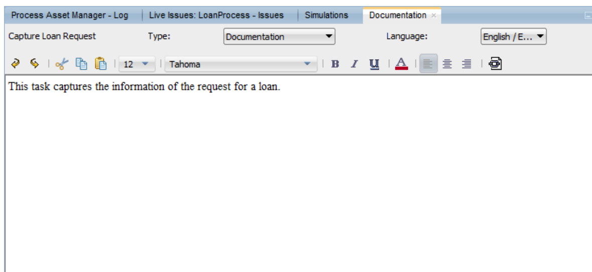
Figure 1-10 Documentation Window
