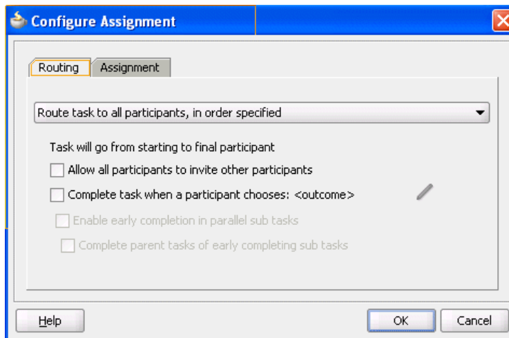
Figure 29-40 Configure Assignment
