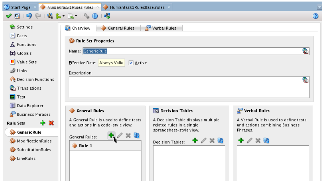
Figure 32-36 Rule-Definition Section
