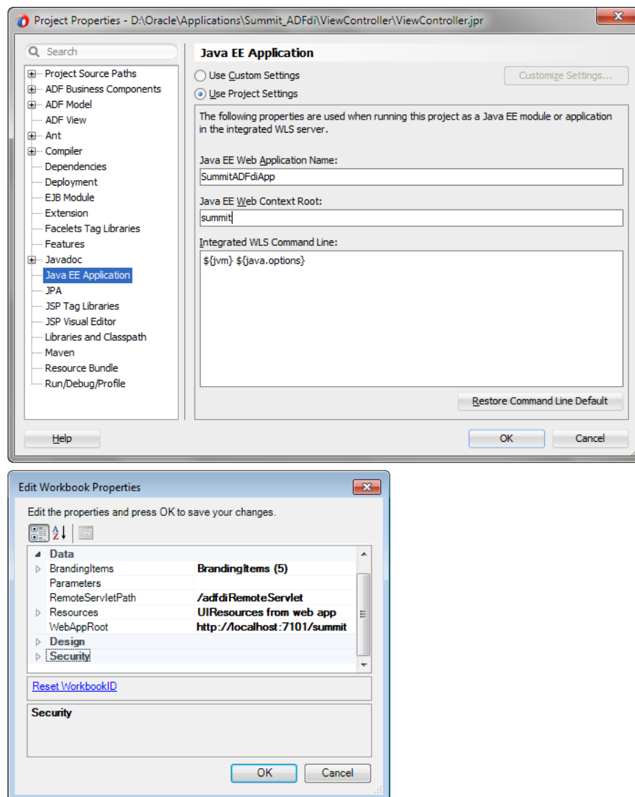
Figure 4-7 Setting Web Context Root in JDeveloper and Integrated Excel Workbook
