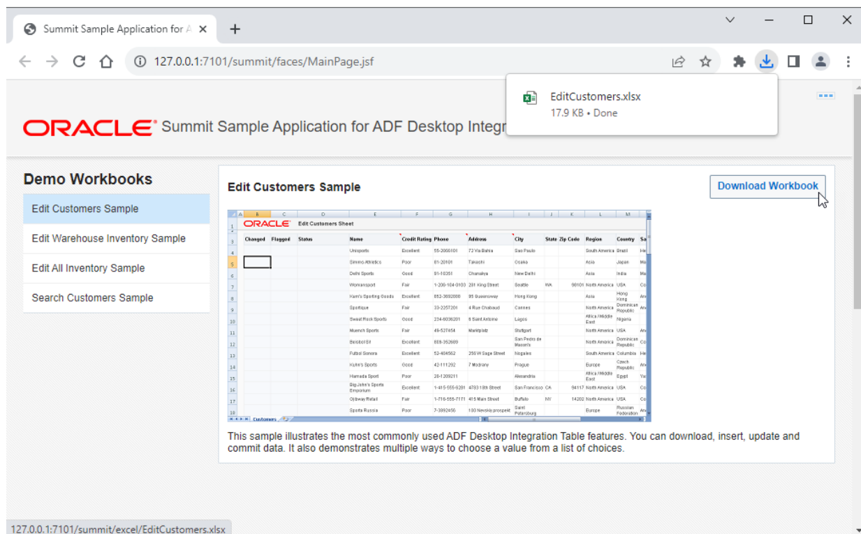
Figure 15-2 Invoking an Integrated Excel Workbook from a Fusion Web Application
