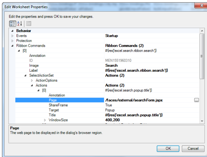
Figure 9-23 Ribbon Command Configured to open a Web Page
