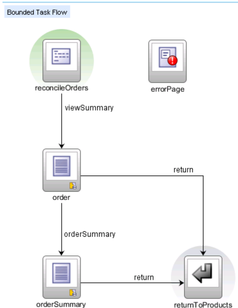
Figure 5-2 ADF Bounded Task Flow
