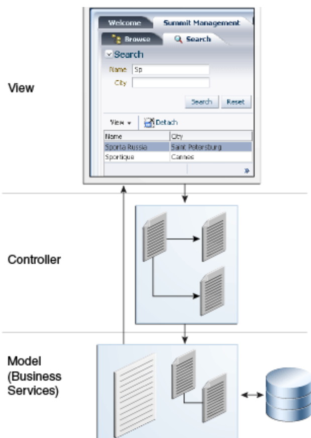
Figure 3-2 Basic MVC Architecture
