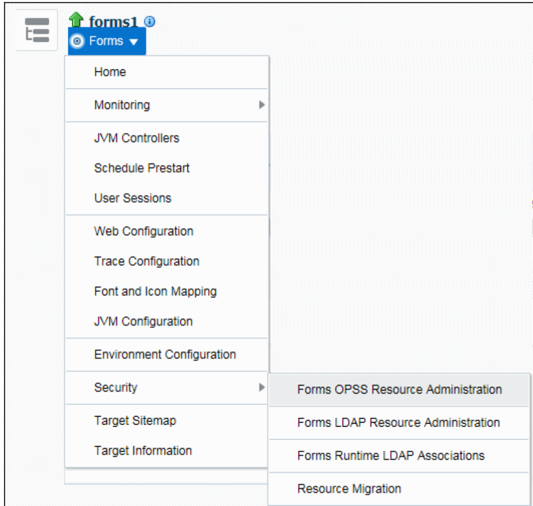
Figure 33 Forms drop-down
