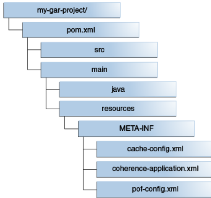
Figure 11-1 Maven Project Files
