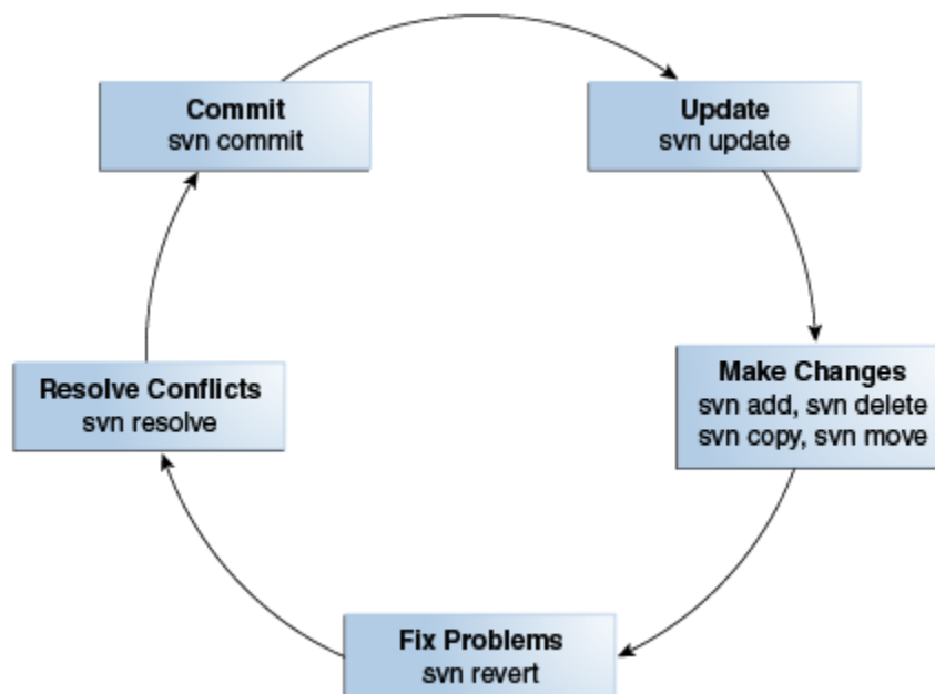
Figure 3-1 SVN Workflow
