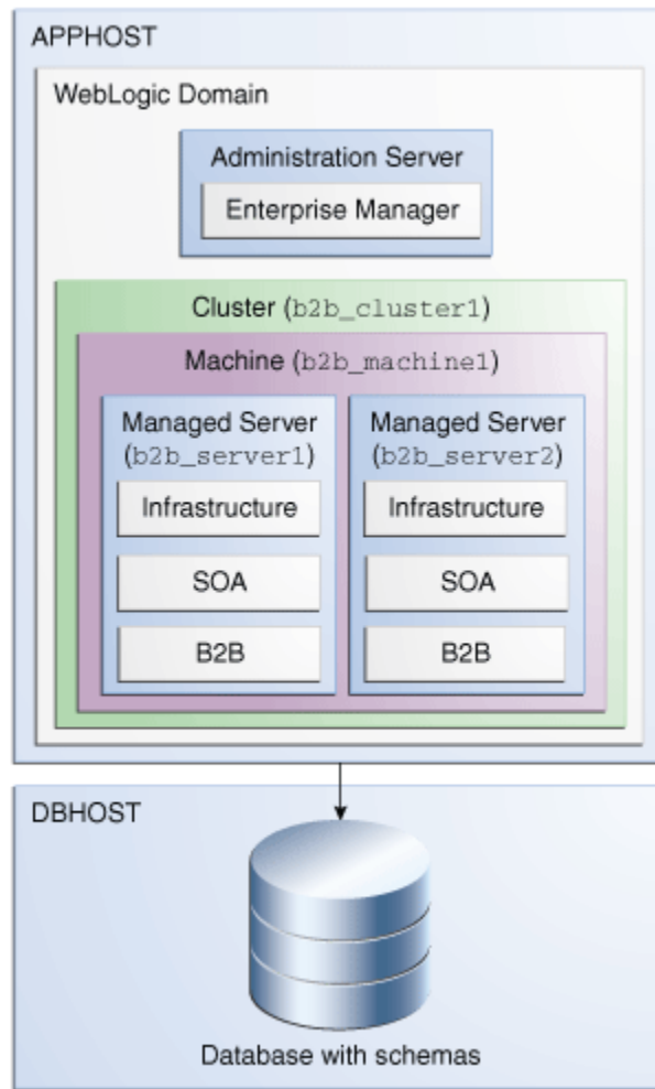
Figure 1-1 Standard Topology for Oracle B2B
