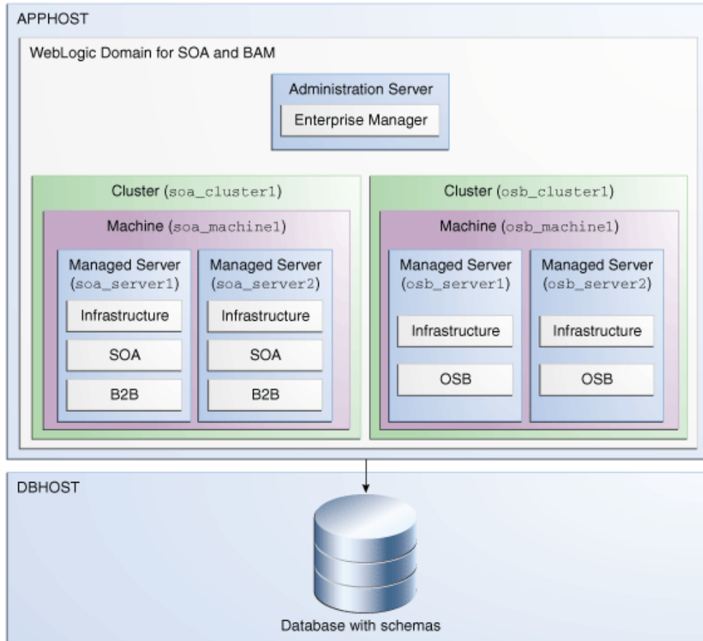
Figure A-2 Roadmap for Installing and Configuring the Oracle SOA Suite, B2B, and Oracle Service Bus Topology
