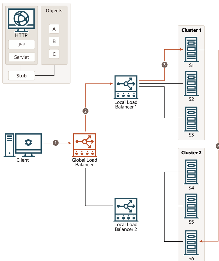
Figure 6-6 MAN Replication
