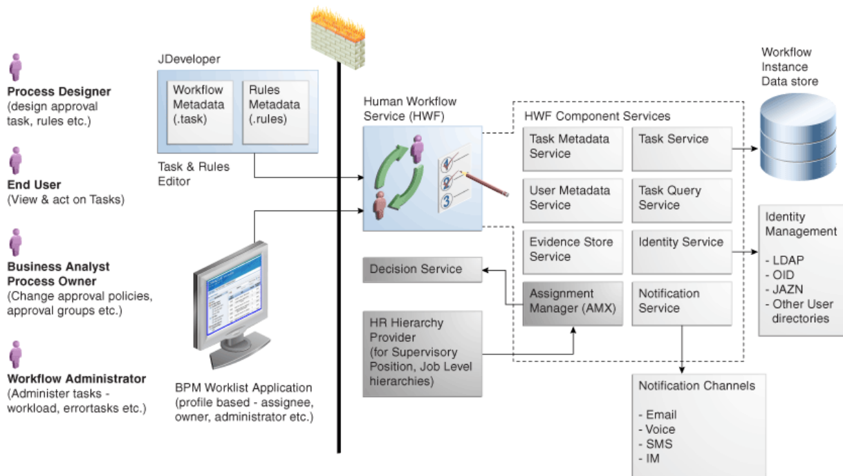
Figure 32-1 Overall Architecture
