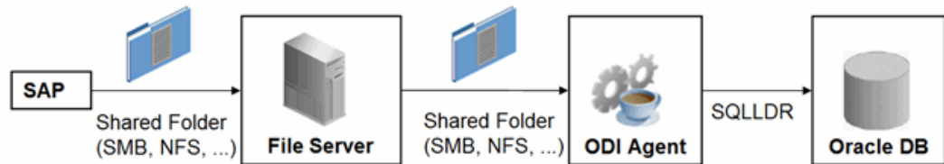
Figure 7-2 Configuration 2
