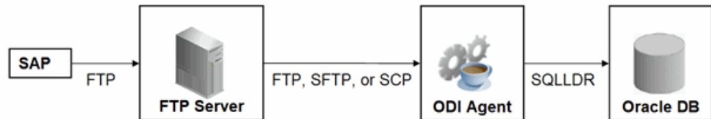
Figure 7-4 Configuration 2: FTP Server is not installed on ODI Agent machine
