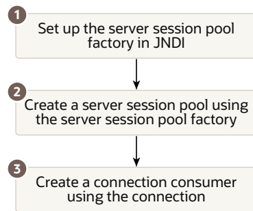
Figure A-2 Preparing for Concurrent Message Processing
