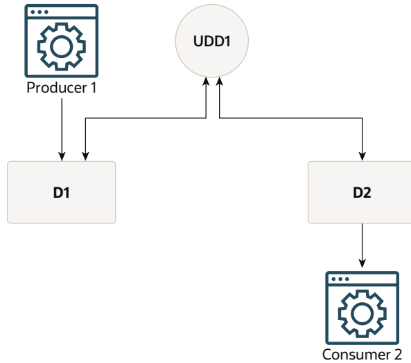
Figure 9-3 Stuck Messages
