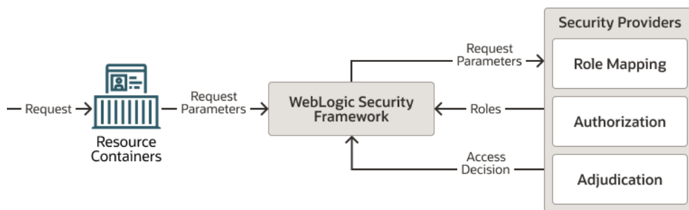
Figure 5-5 Authorization Process
