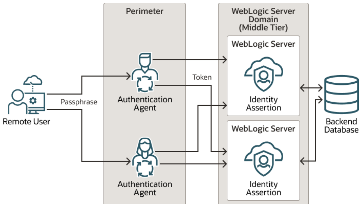
Figure 3-2 Perimeter Authentication
