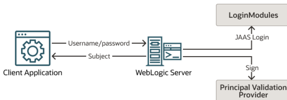
Figure 5-4 The Principal Validation Process
