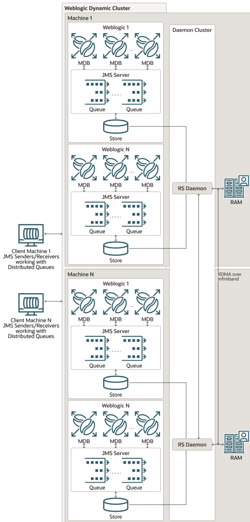
Figure 3-1 Clustered Replicated Store
