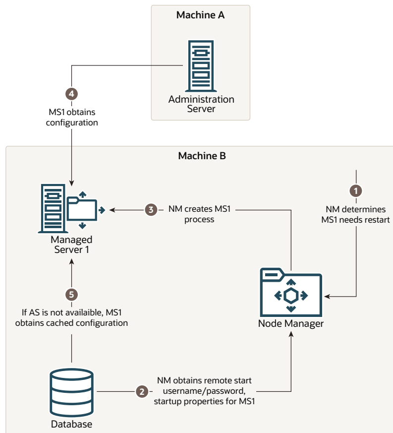
Figure 1-5 Restarting a Managed Server
