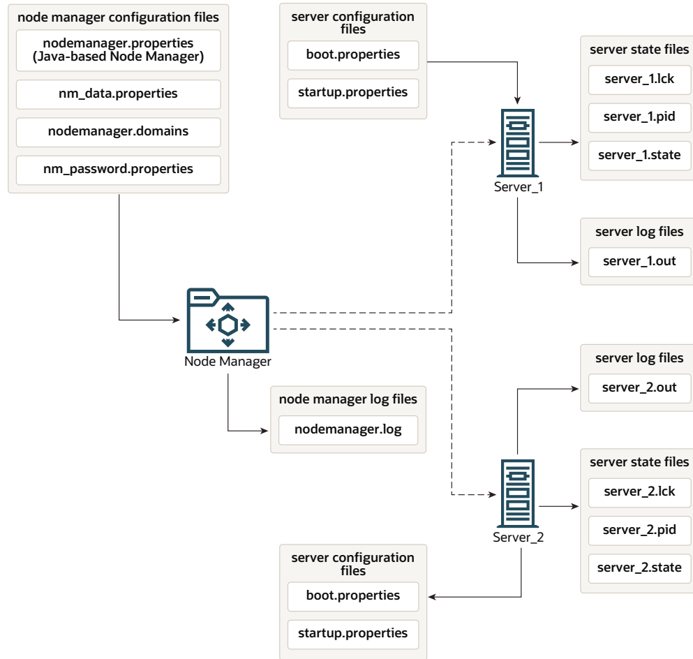
Figure 1-7 Node Manager Configuration and Logging Environment
