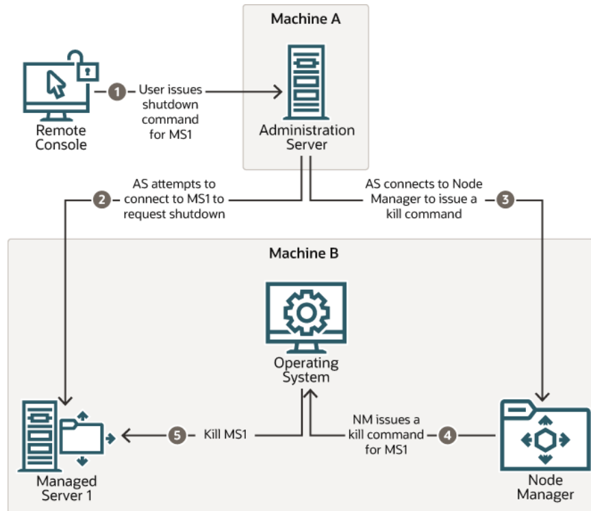
Figure 1-6 Shutting Down a Server Instance Under Node Manager Control
