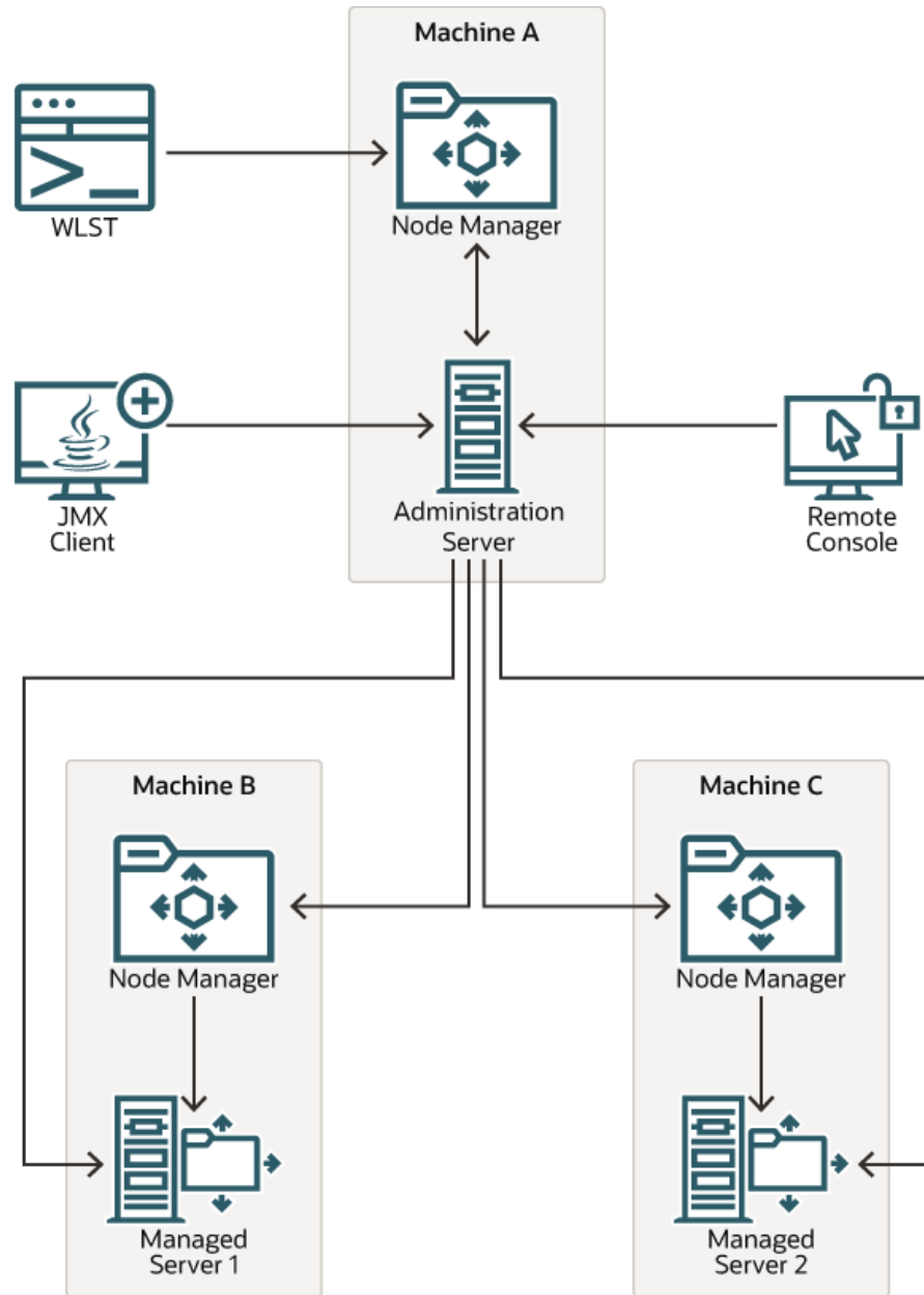
Figure 1-1 Node Manager in the Oracle WebLogic Server Environment
