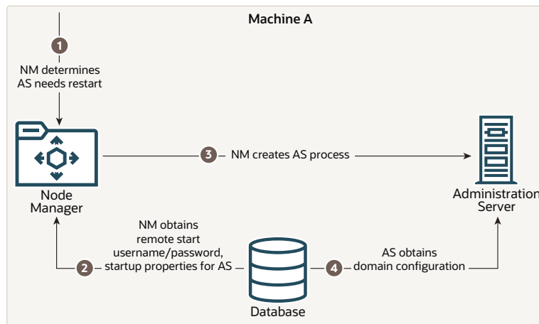
Figure 1-4 Restarting an Administration Server
