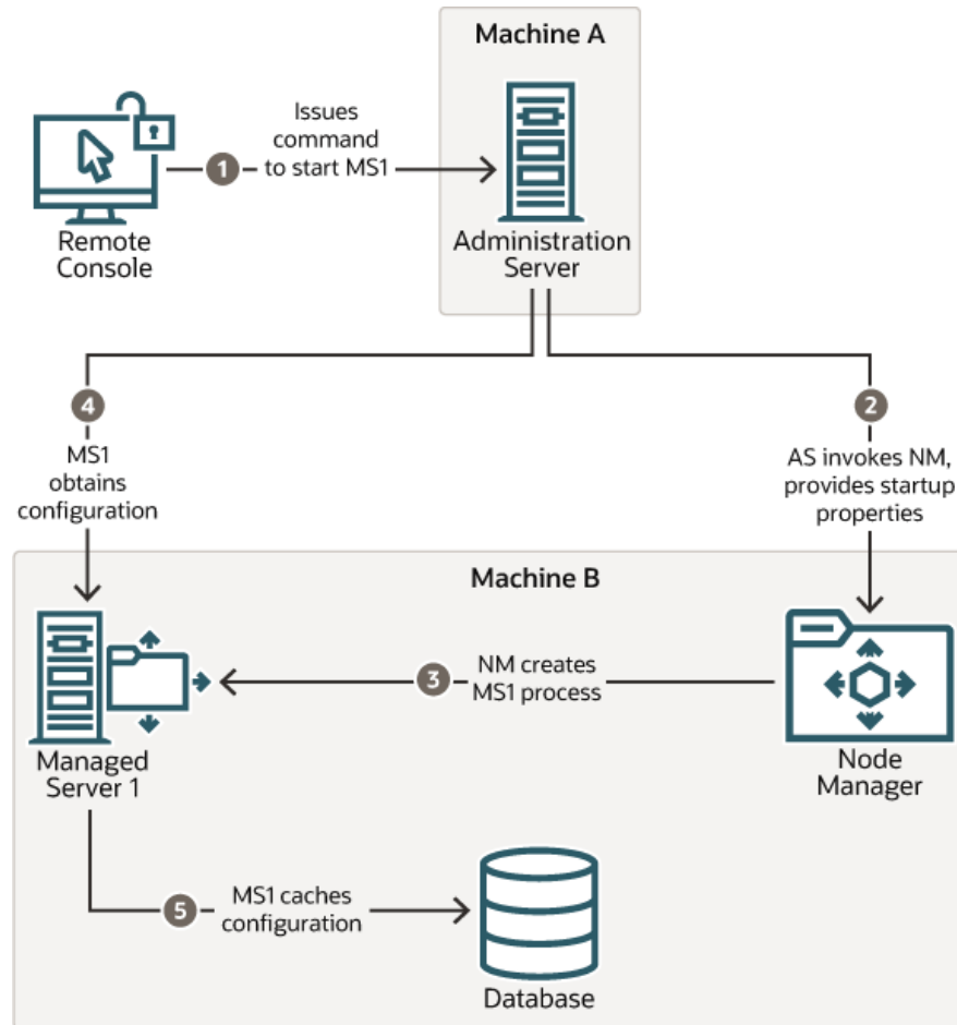
Figure 1-3 Starting a Managed Server
