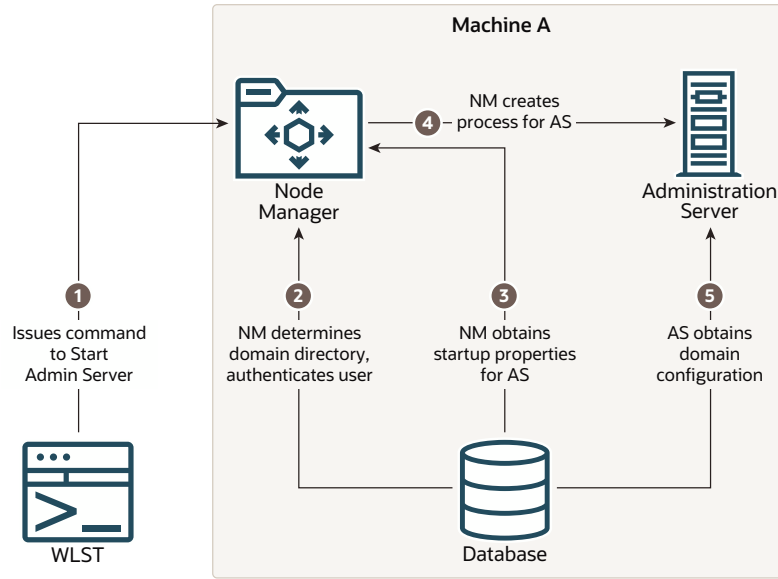
Figure 1-2 Starting an Administration Server
