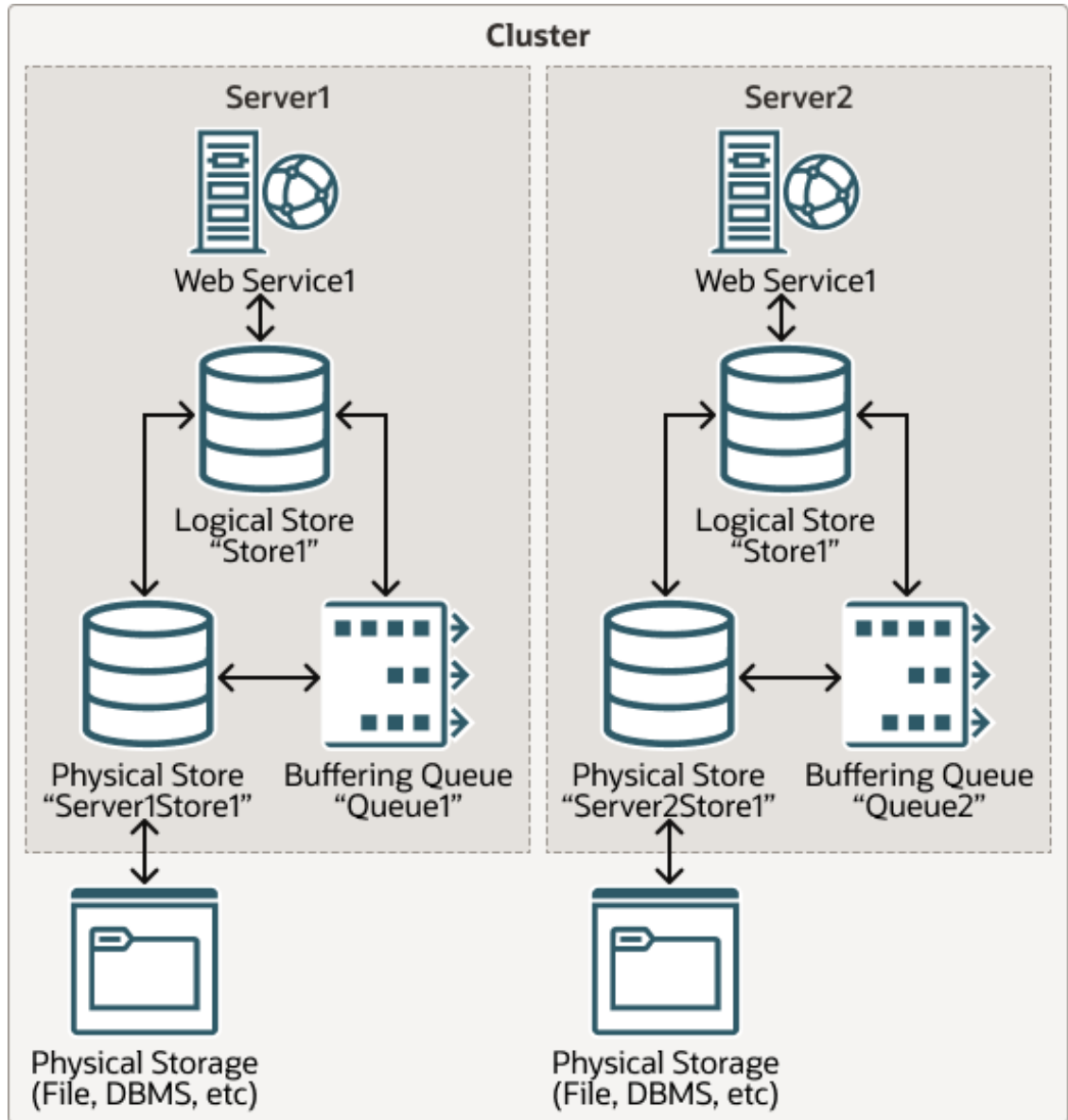
Figure 21-1 Example Web Service Persistence Configuration
