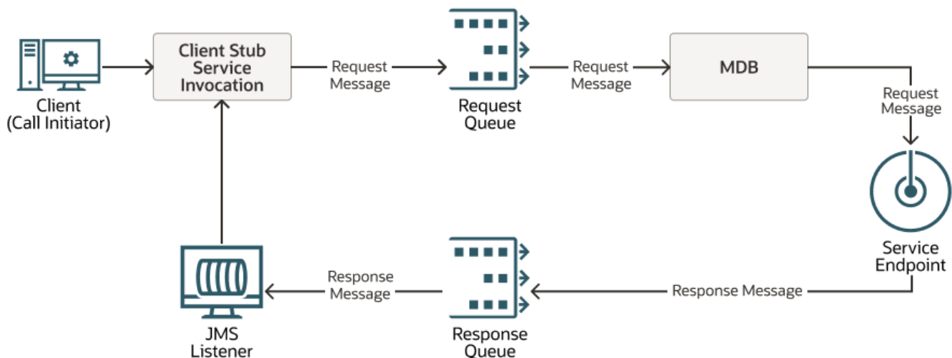
Figure 17-1 Web Service Invocation Using SOAP Over JMS Transport
