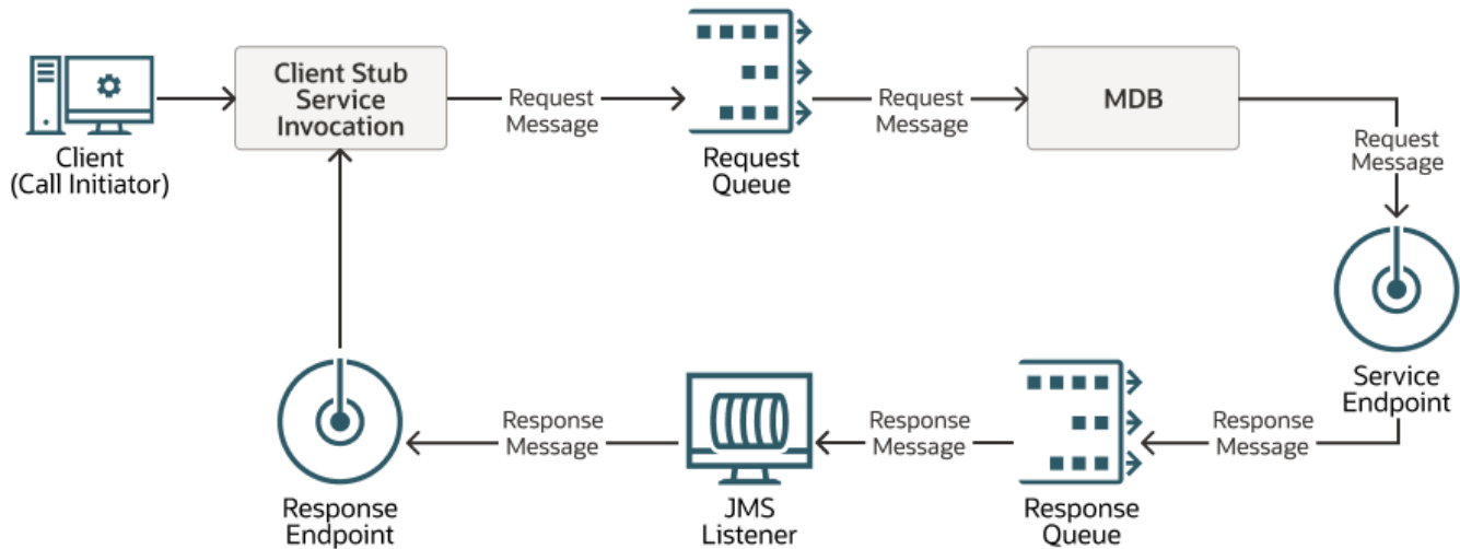
Figure 17-2 Asynchronous Web Service Invocation Using SOAP Over JMS Transport
