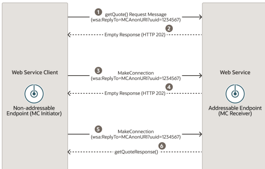
Figure 12-2 Make Connection Message Flow
