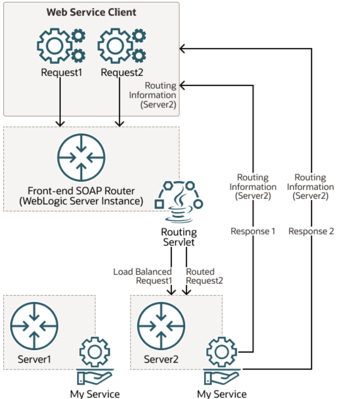
Figure 23-2 Routing Web Service Requests to a Single Server
