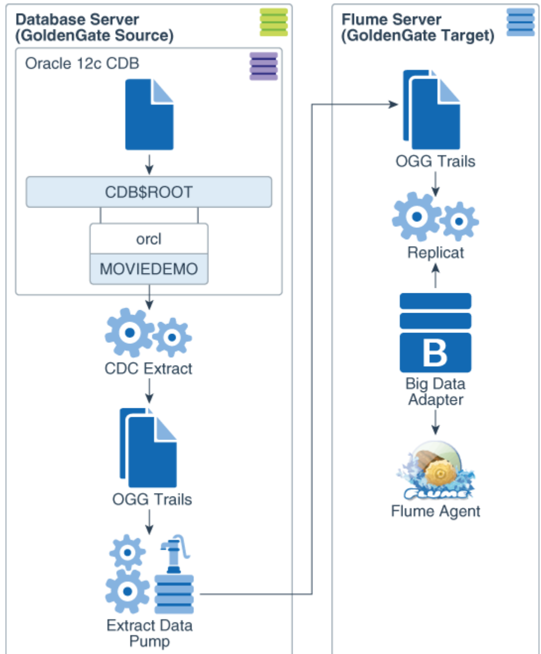
Figure 6-2 Oracle GoldenGate Deployment
