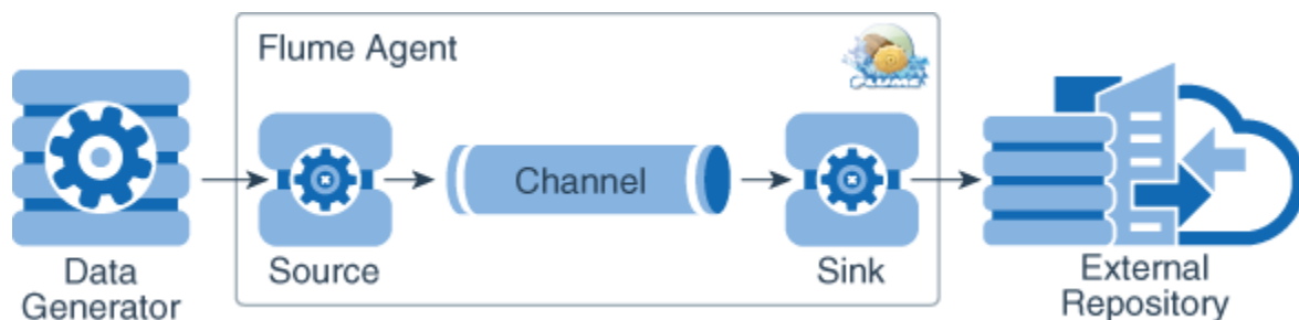
Figure 6-1 Flume Agent Architecture
