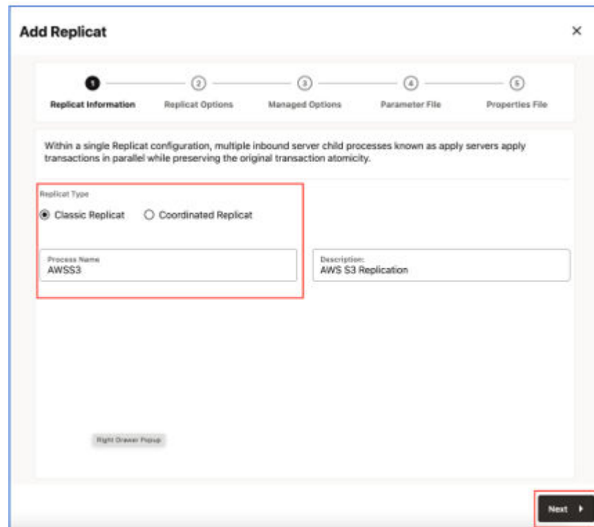
Figure 8-21 Add Replicat
