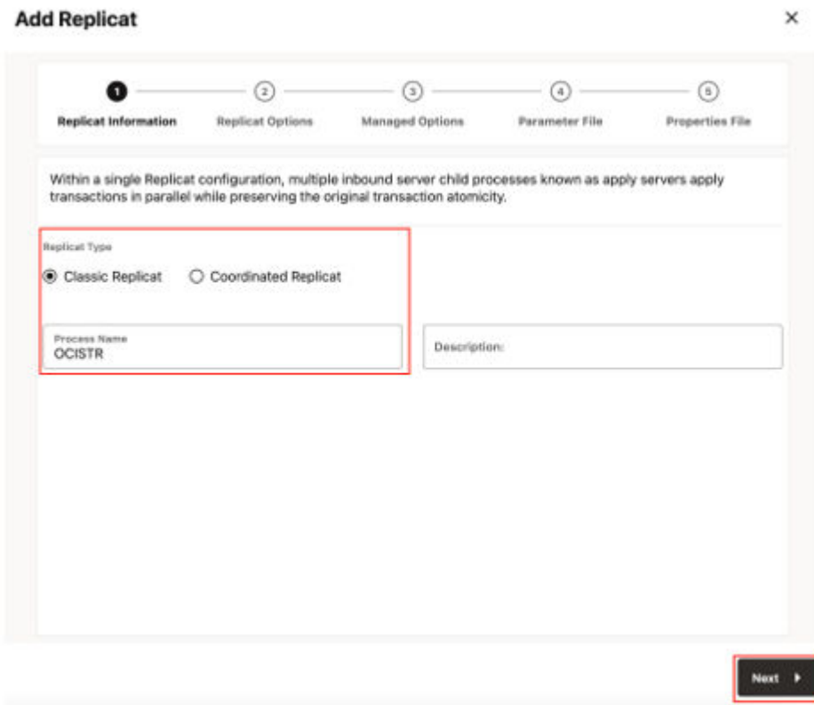
Figure 8-45 Add Replicat
