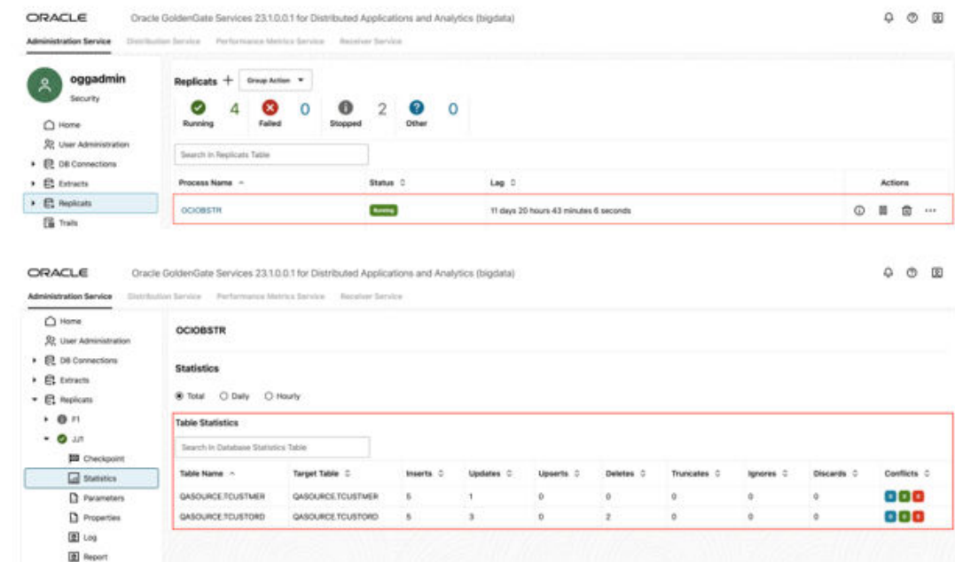
Figure 8-41 Replication Statistics
