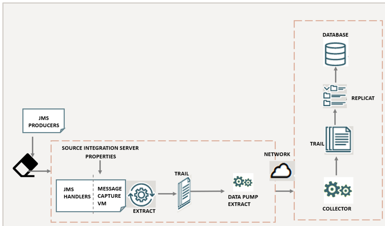
Figure 9-3 Configuration for JMS Message Capture
