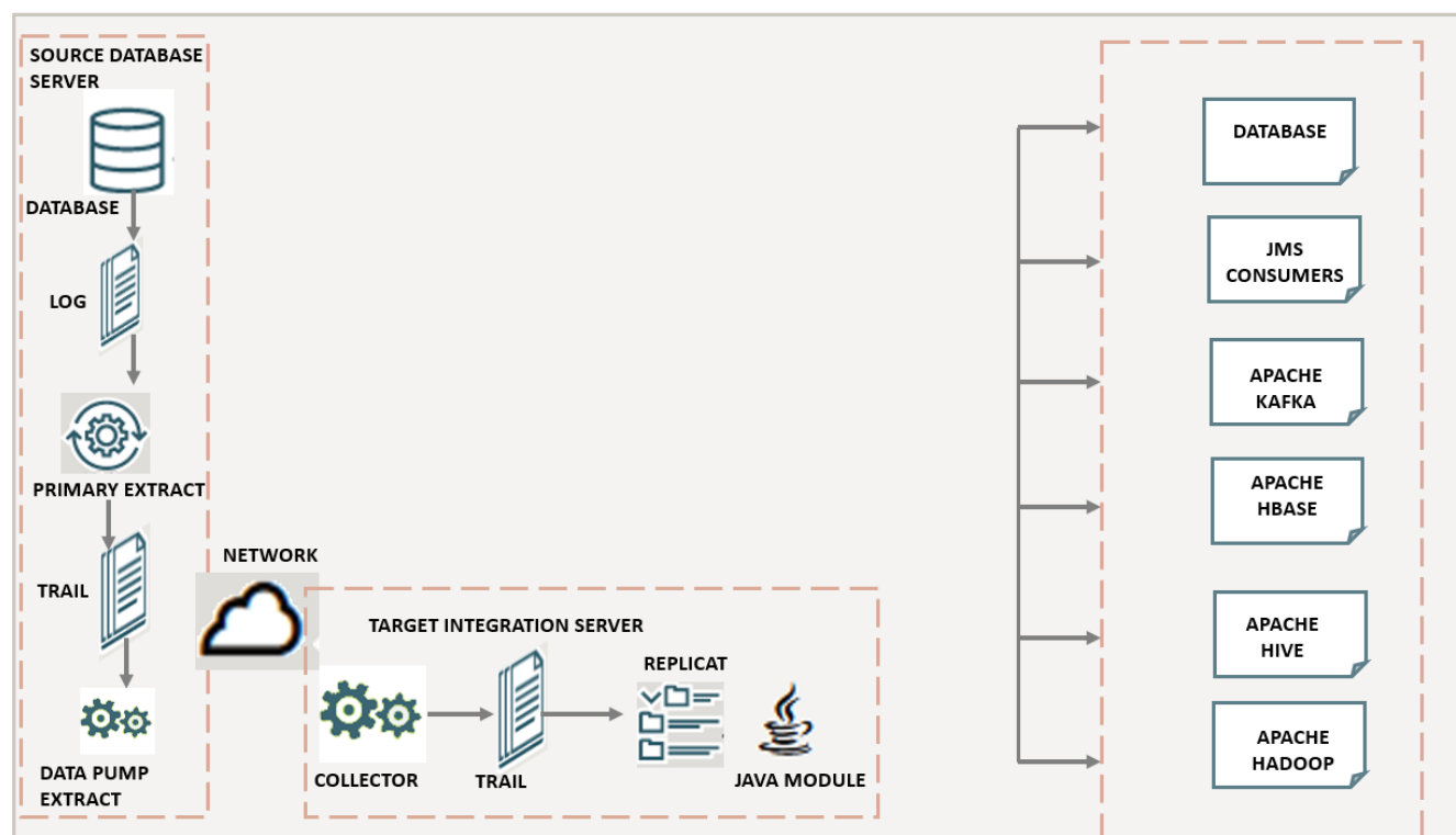
Figure 9-1 Configuration for Delivering JMS Messages
