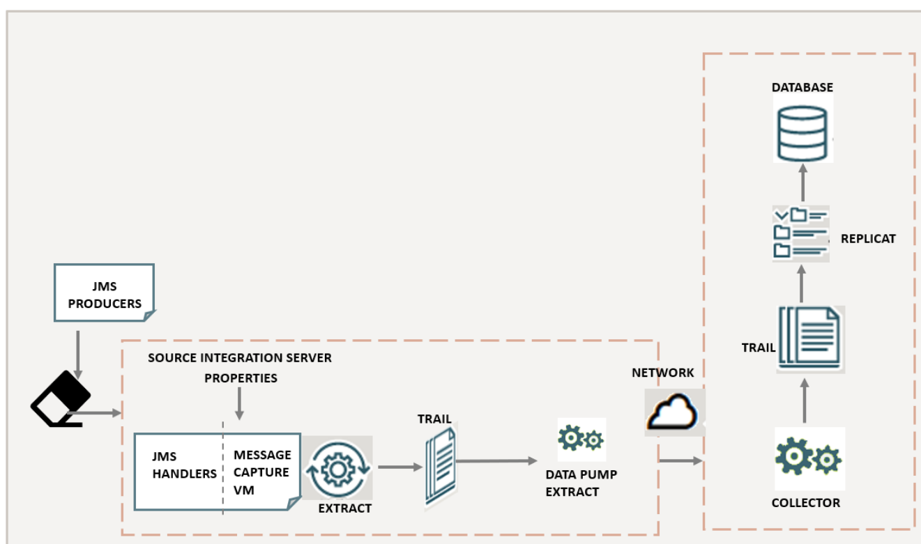
Figure 9-2 Configuration for JMS Message Capture
