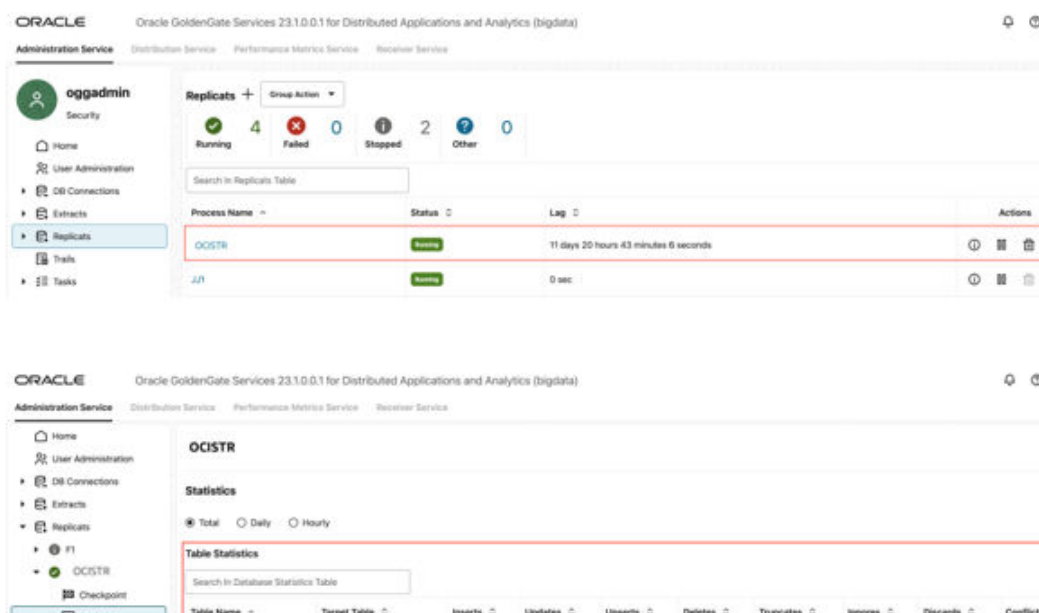
Figure 8-49 Replicat Statistics
