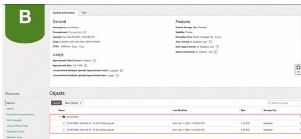
Figure 8-42 OCI Console
