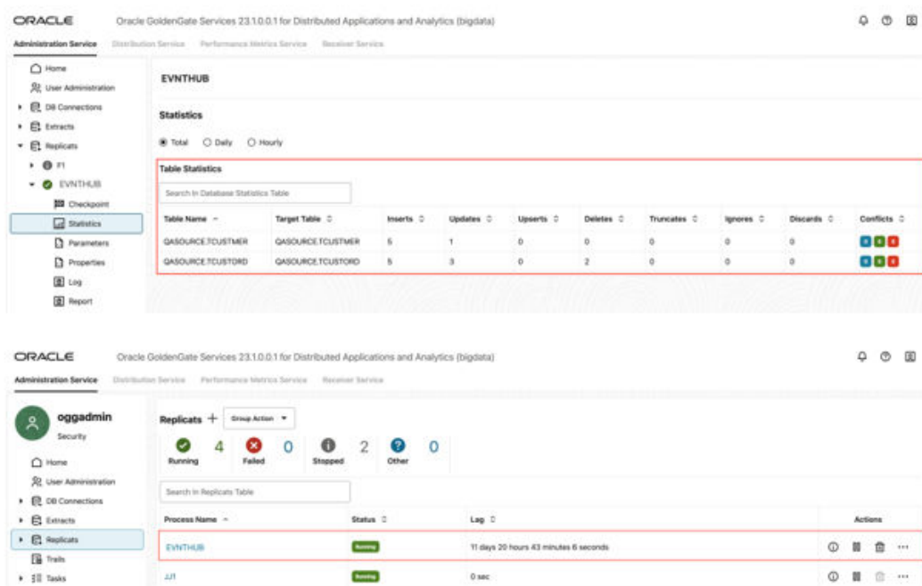
Figure 8-57 Replicat Statistics
