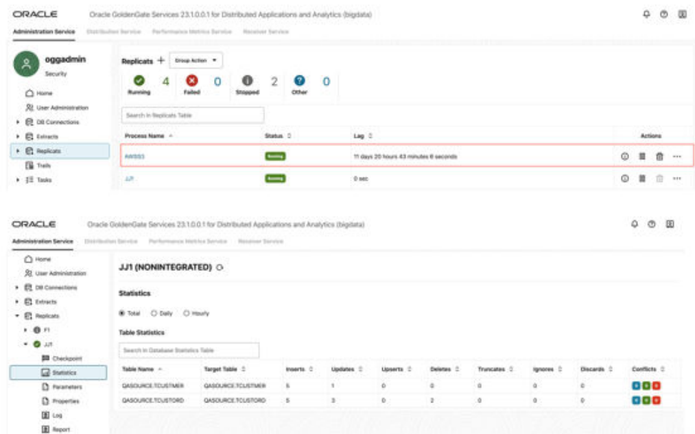
Figure 8-25 Replication Statistics
