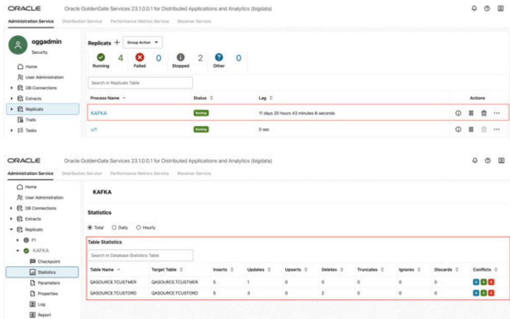
Figure 8-81 Replicat Statistics
