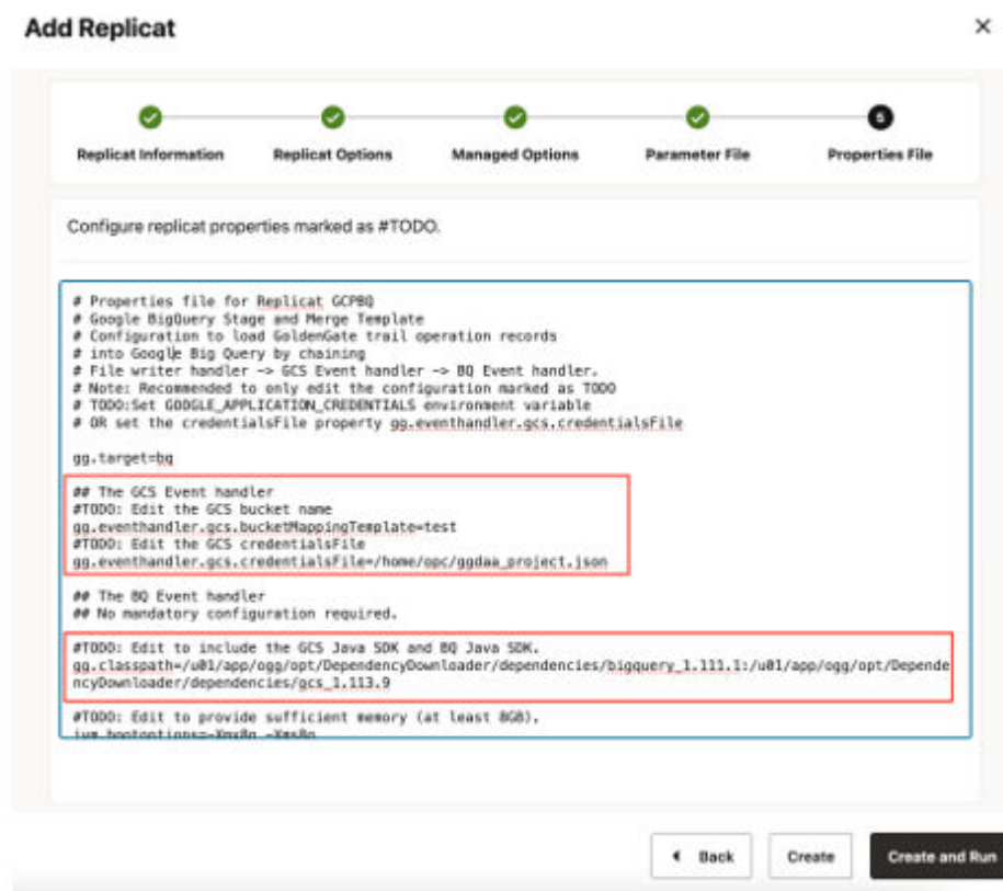
Figure 8-65 Properties File
