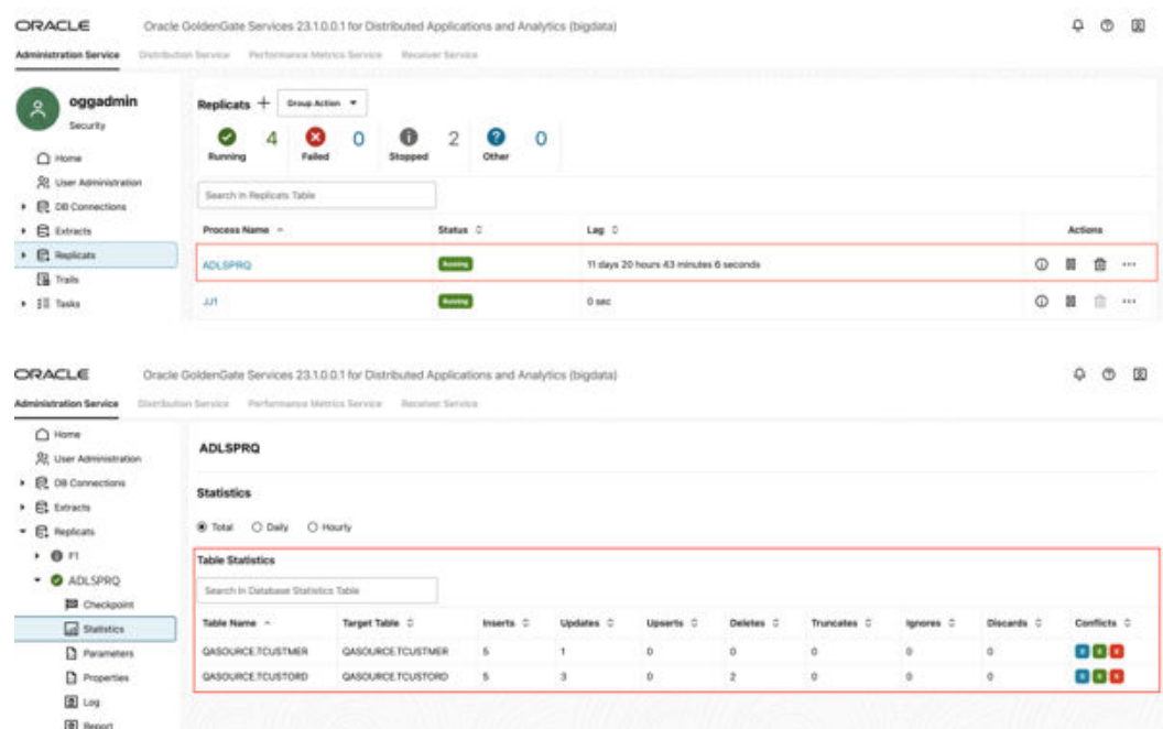
Figure 8-33 Replicats Statistics
