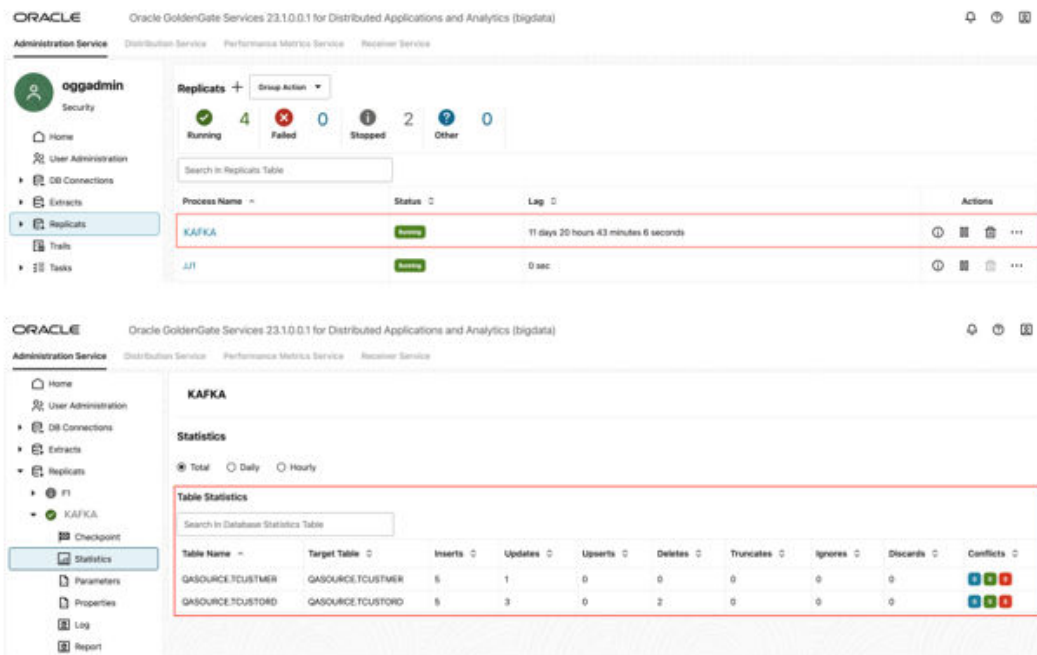
Figure 8-81 Replicat Statistics
