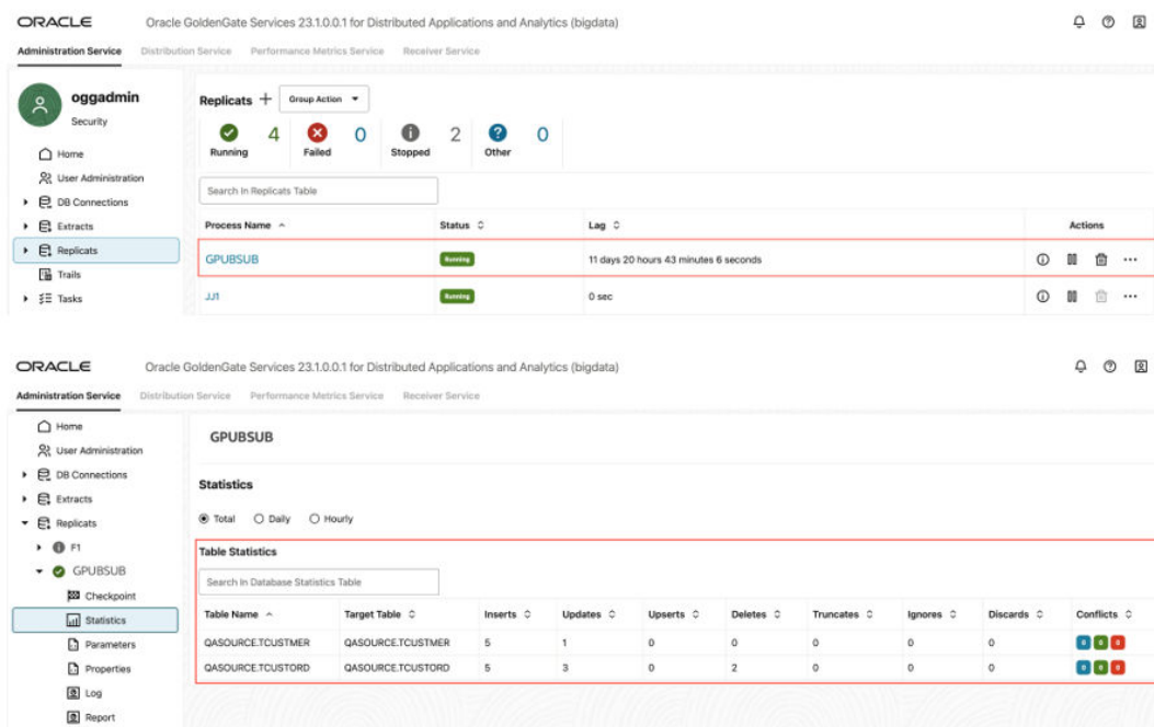
Figure 8-74 Replication Statistics
