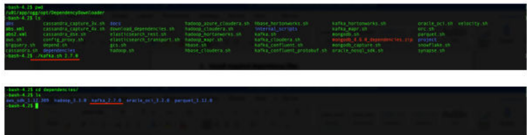
Figure 8-43 Execute kafka.sh
