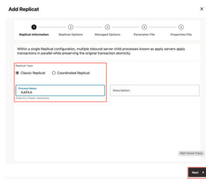
Figure 8-77 Add Replicat
