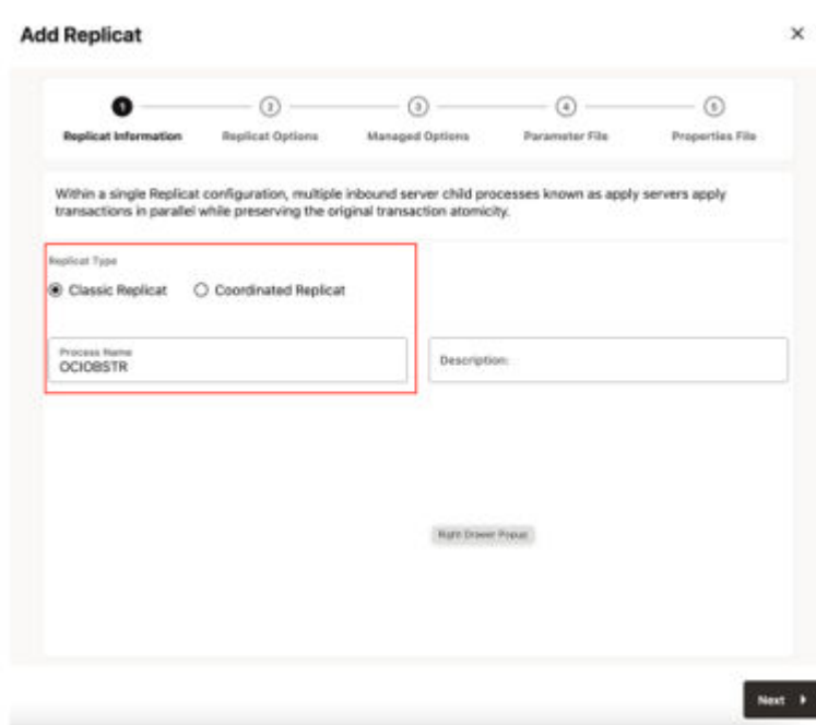
Figure 8-37 Add Replicat
