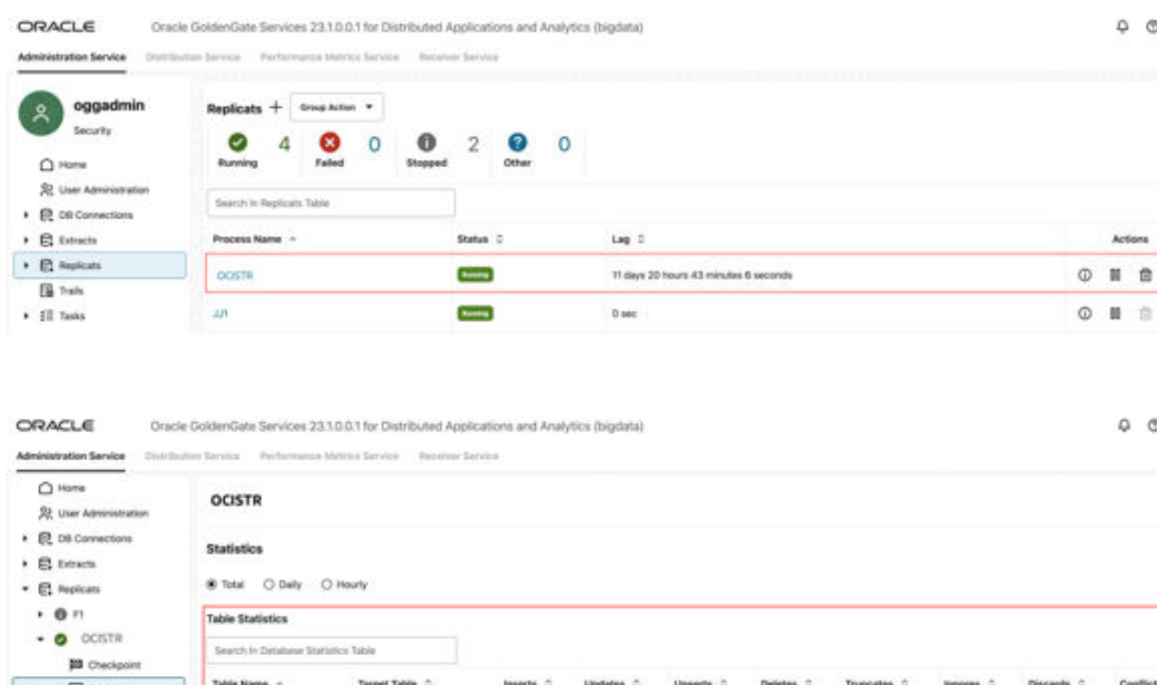
Figure 8-49 Replicat Statistics
