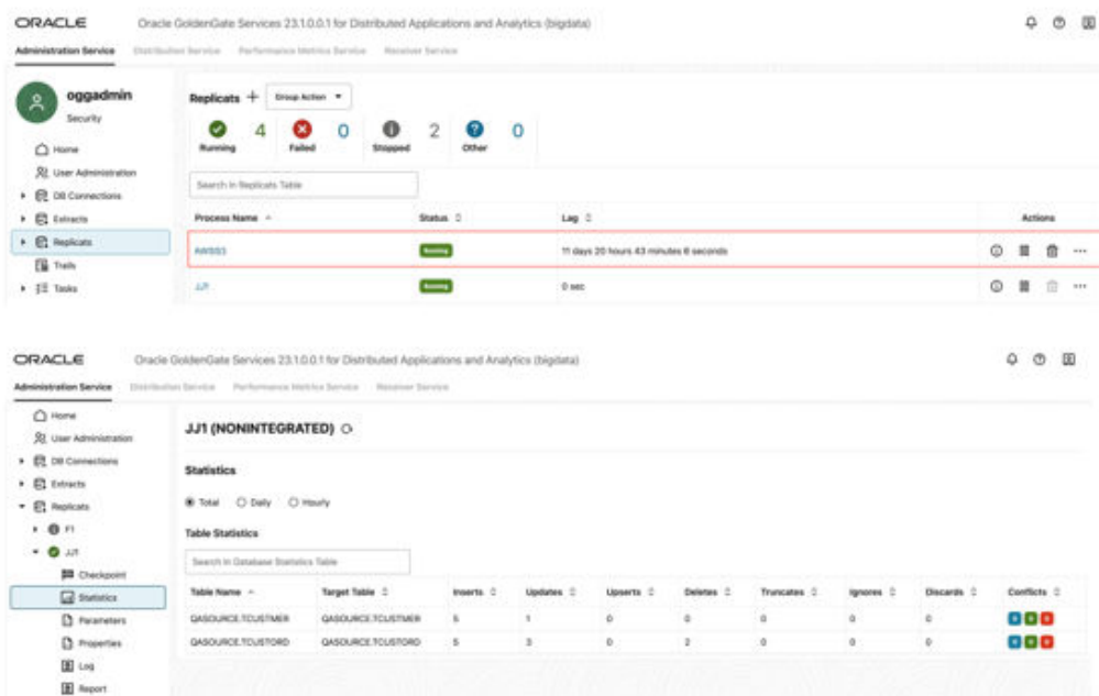
Figure 8-25 Replication Statistics
