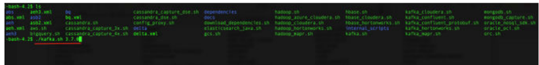
Figure 8-51 Execute kafka.sh
