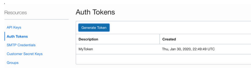
Figure 9-7 Auth-Tokens
