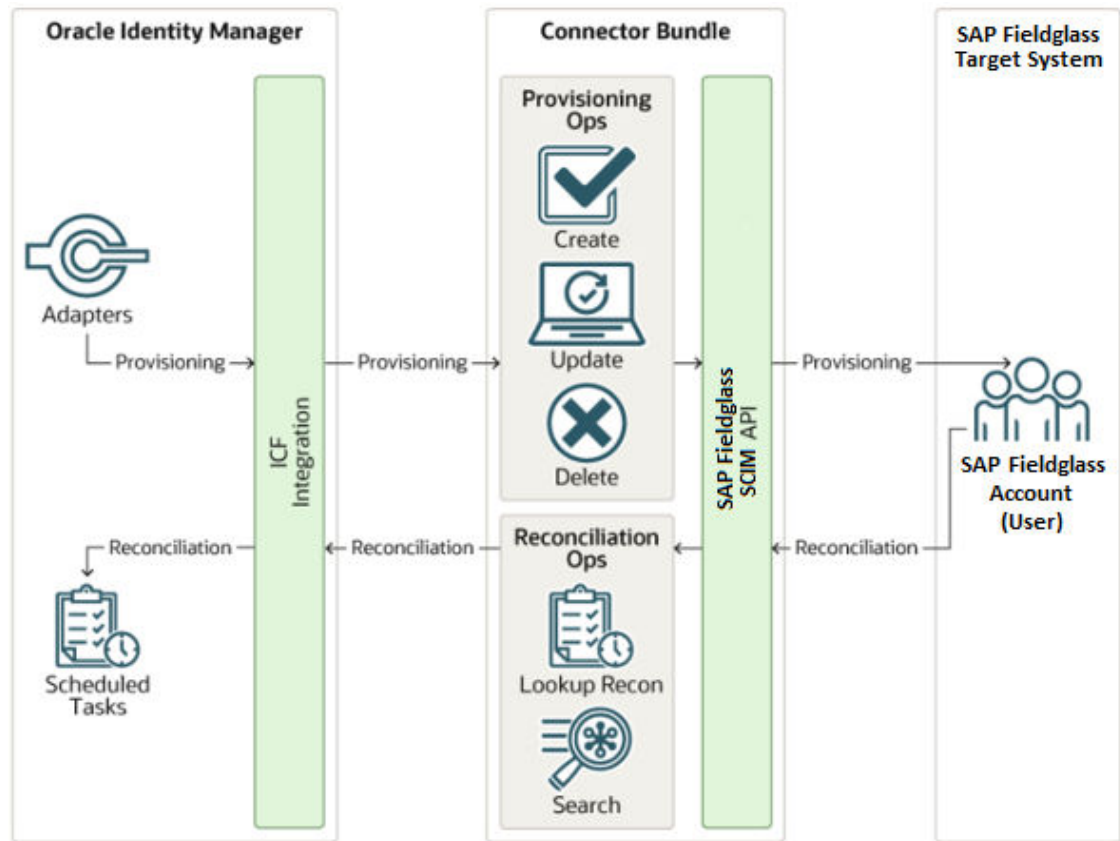
Figure 1-1 Architecture of the SAP Fieldglass Connector
