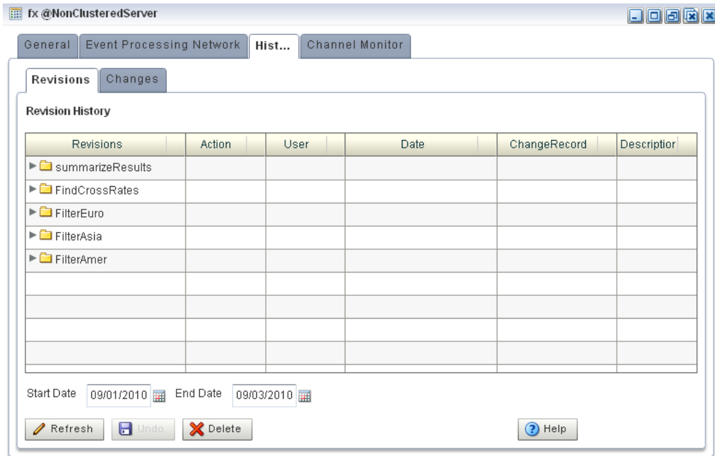
Figure 7-1 History Tab
