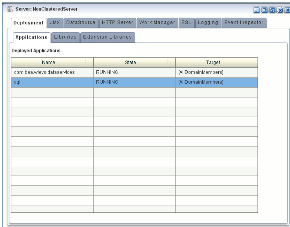
Figure 9-1 Applications Tab
