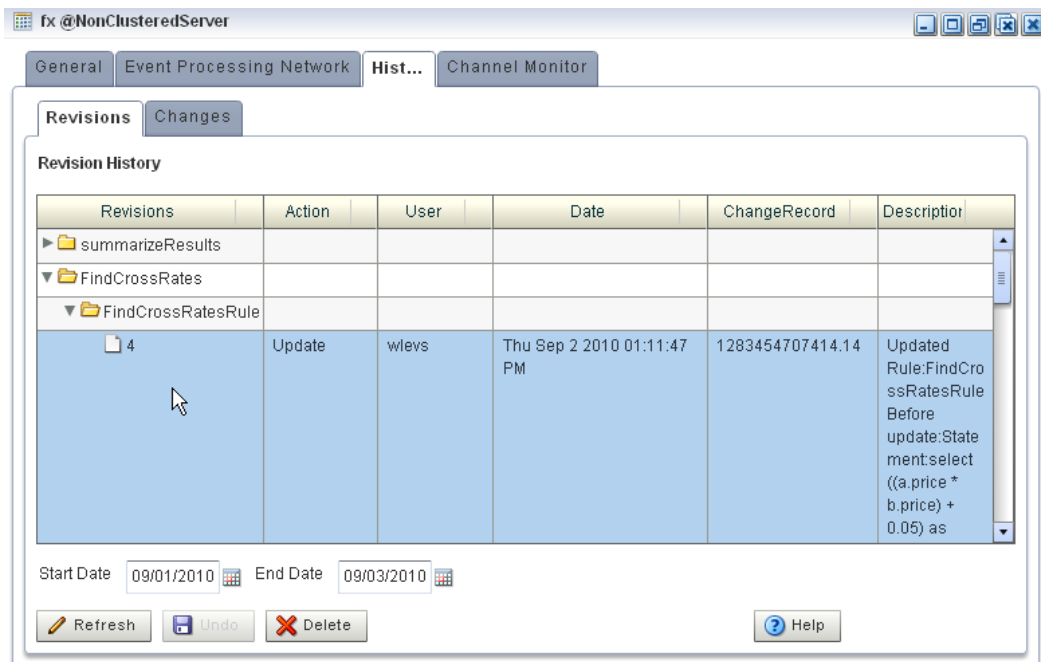
Figure 7-2 Revisions Tab
