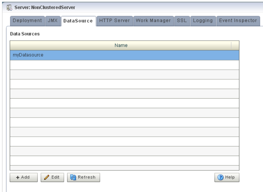
Figure 12-1 DataSource Tab
