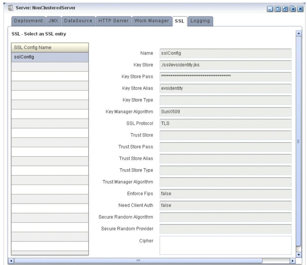
Figure 24-1 SSL Tab
