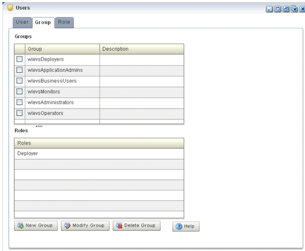
Figure 21-1 Group Tab
