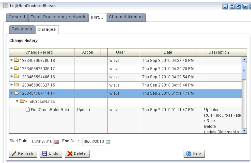
Figure 7-4 Changes Tab
