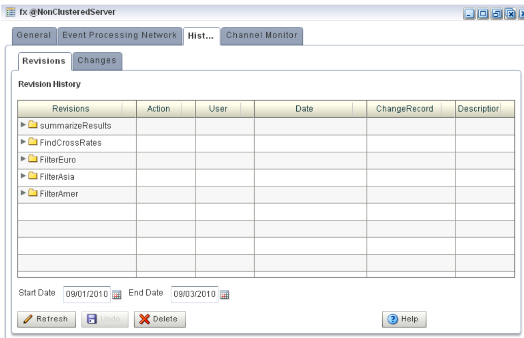
Figure 7-3 History Tab
