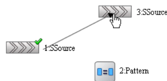
Figure 6-4 Invalid Connection
