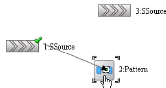
Figure 6-3 Valid Connection
