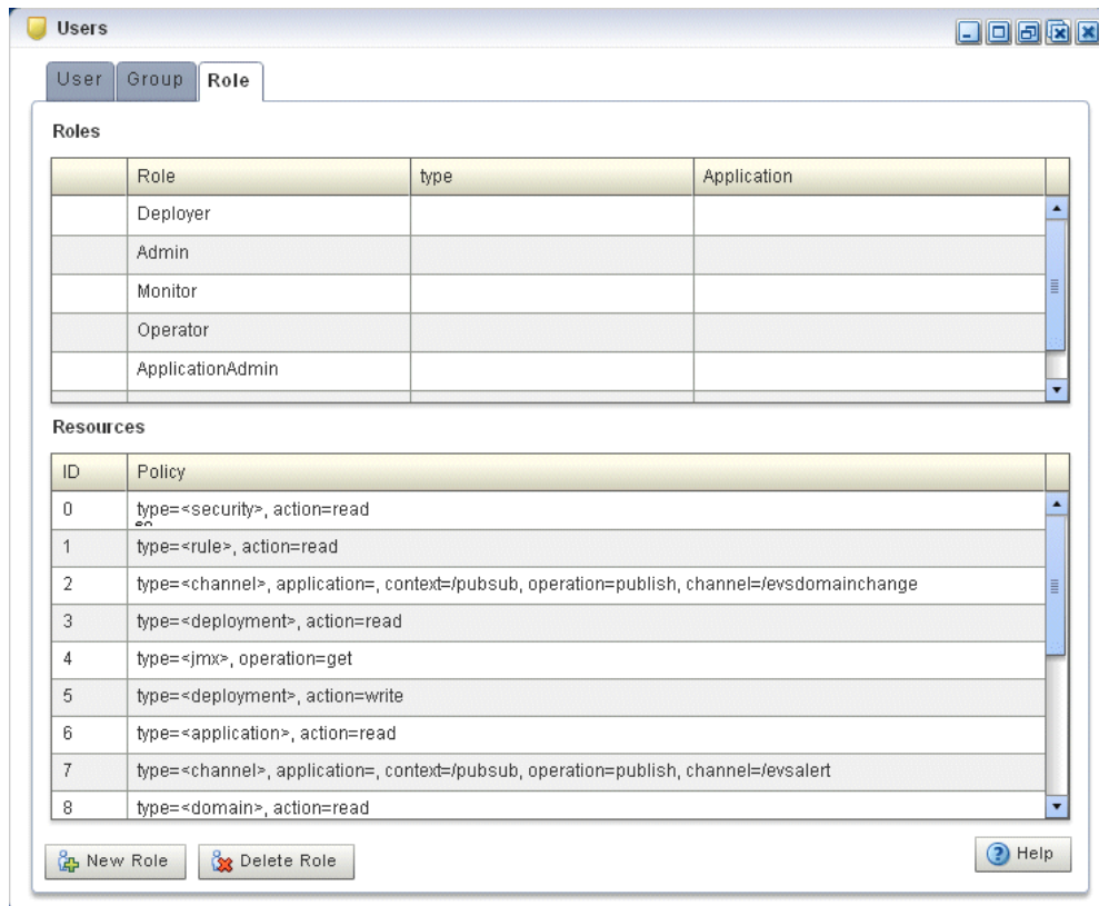
Figure 22-1 Role Tab
