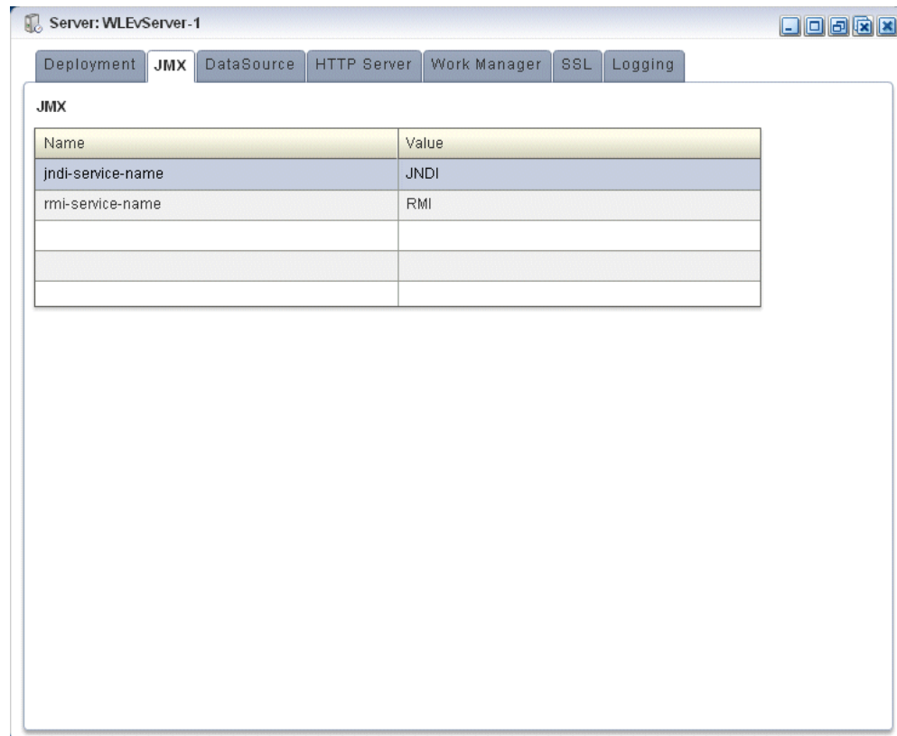
Figure 11-1 JMX Tab
