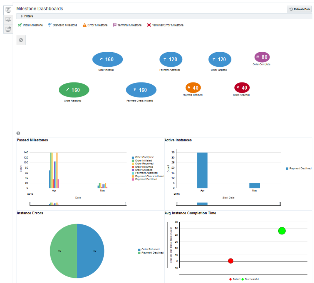
Figure 4-11 View of Milestone Dashboards page when the Preference is set to Combined
