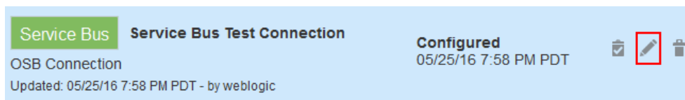
Figure 6-2 Edit Connection
