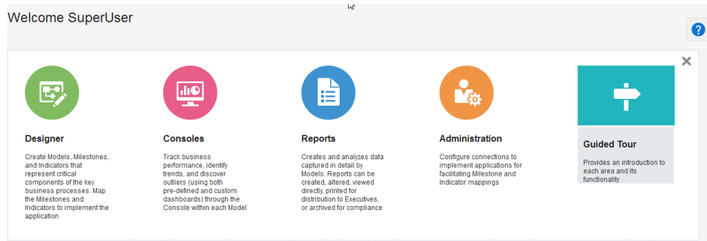
Figure 2-1 Welcome Panel
