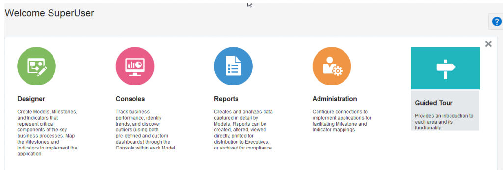
Figure 1-2 Welcome Panel
