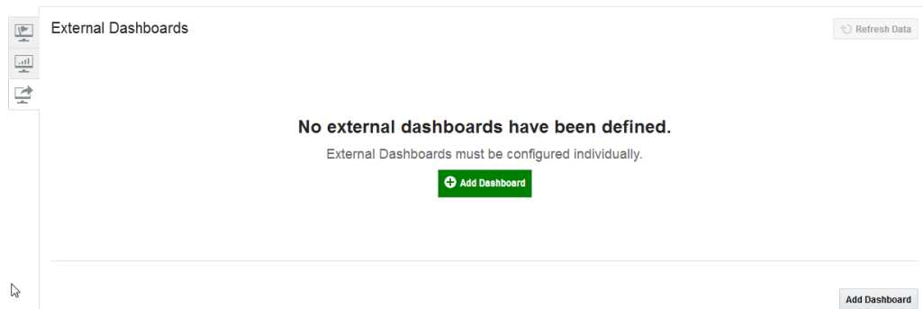
Figure 4-20 External Dashboard
