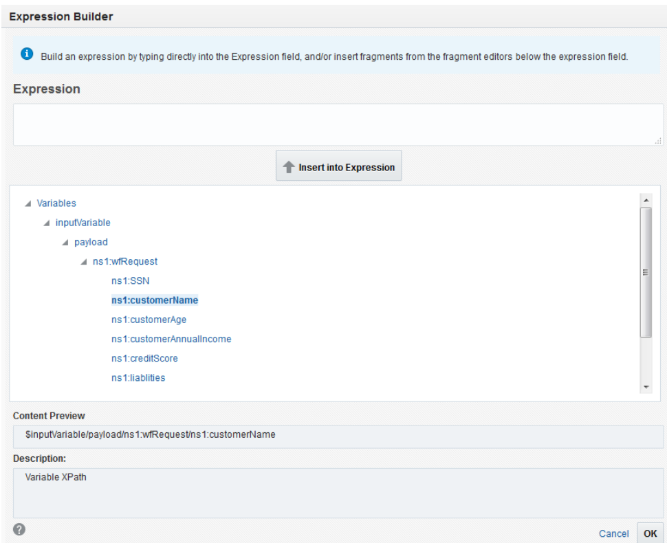
Figure 3-15 Expression Builder
