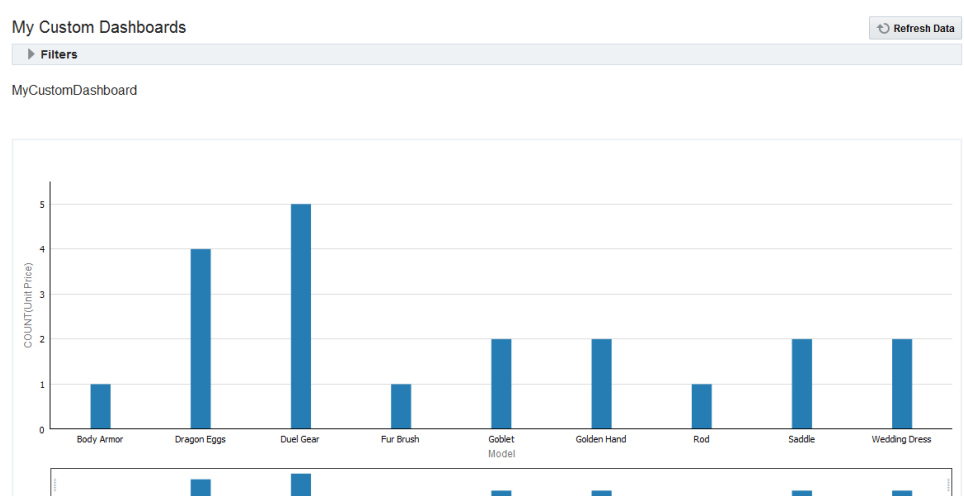
Figure 4-13 Custom Dashboard
