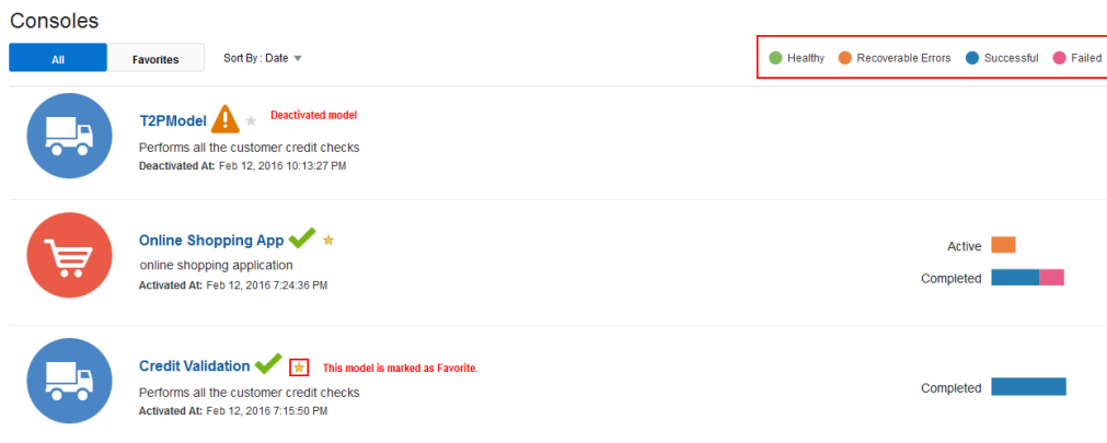
Figure 4-1 Consoles Page
