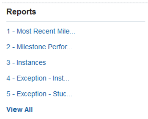
Figure 2-4 Reports Card
