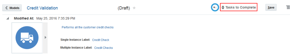
Figure 3-2 Draft Model
