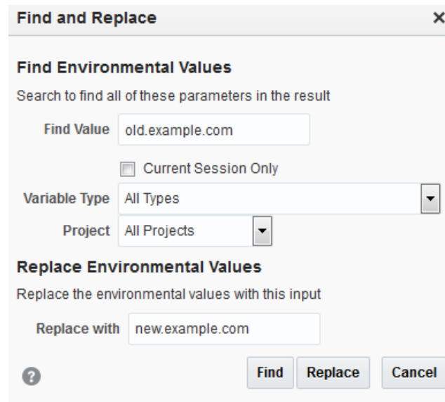
Figure 10-2 Find and Replace Dialog with Replacement Value
