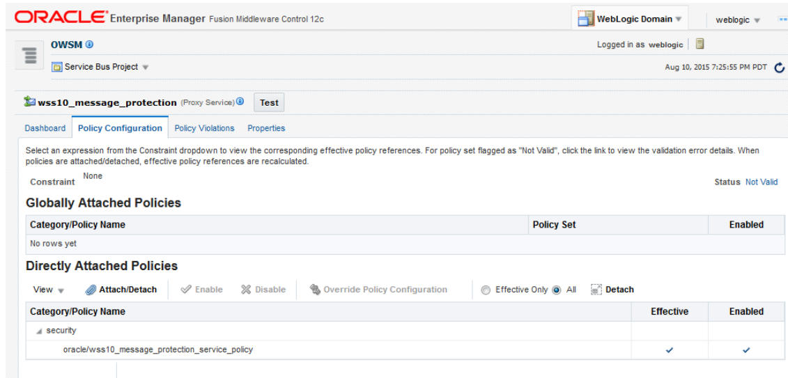
Figure 14-1 Proxy Service Policies Page
