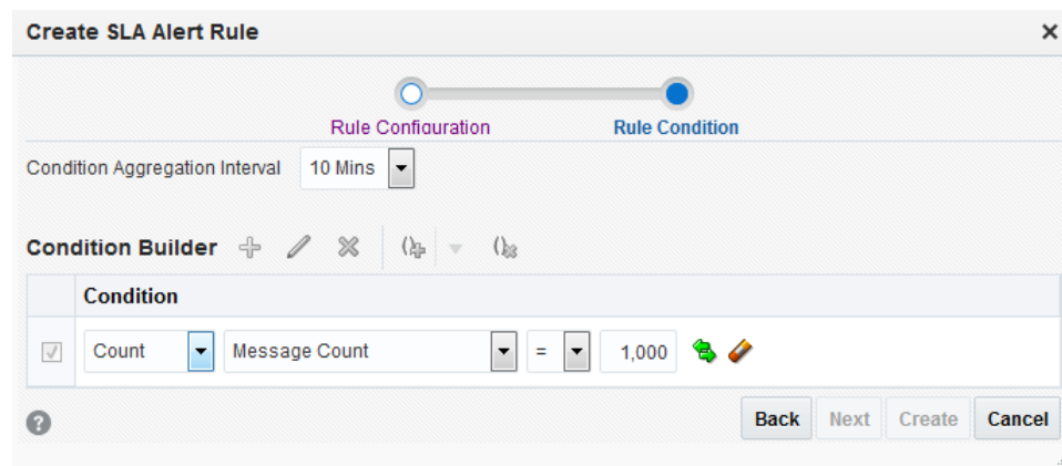
Figure 4-2 Create SLA Alert Rule Wizard - Rule Condition
