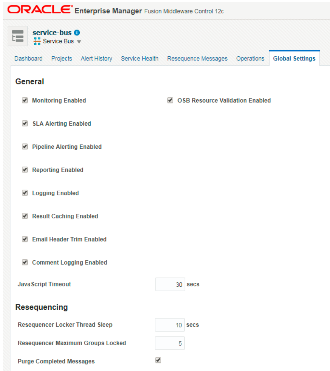
Figure 9-1 The Global Settings Tab
