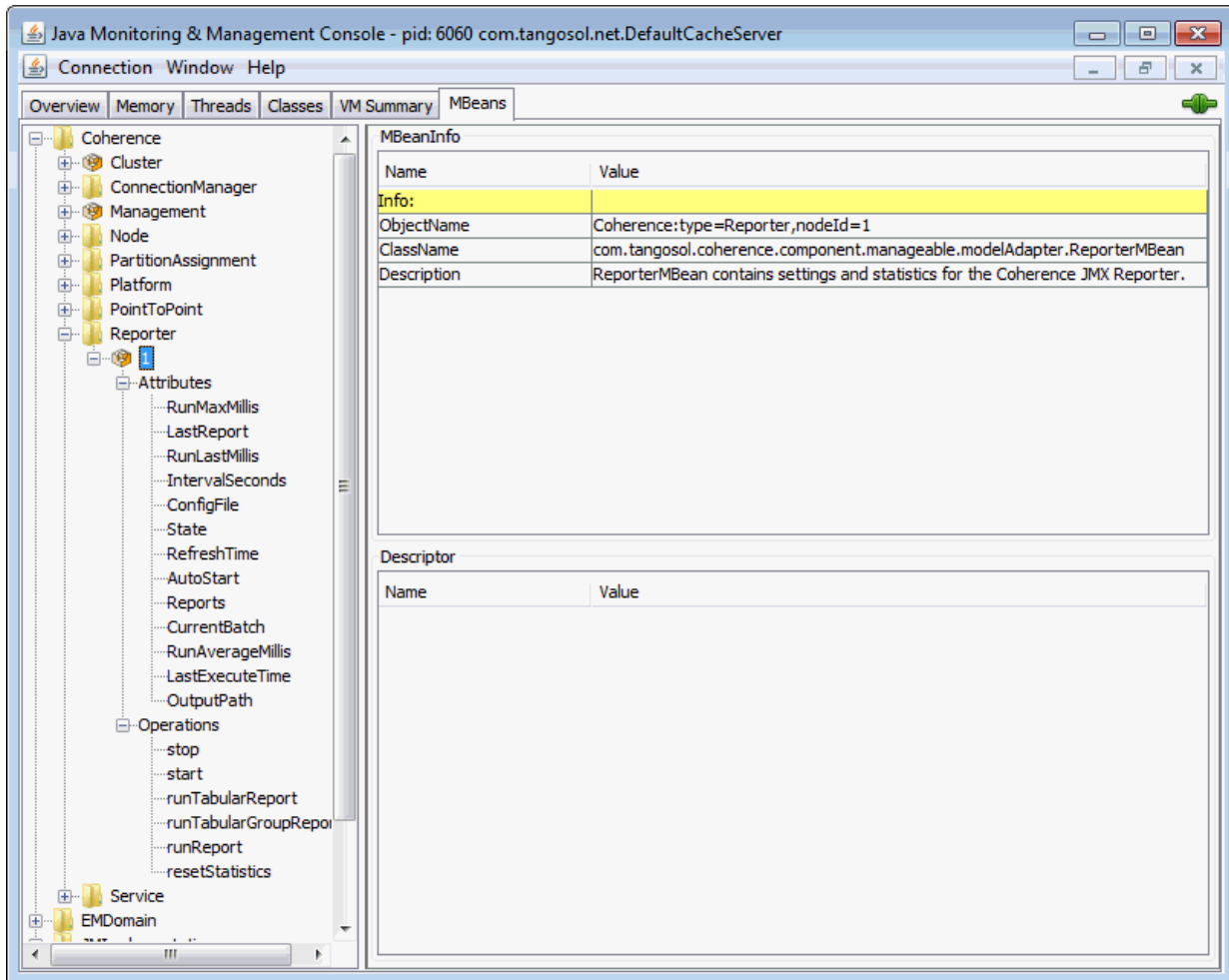
Figure 5-1 ReporterMBean MBean in JConsole
