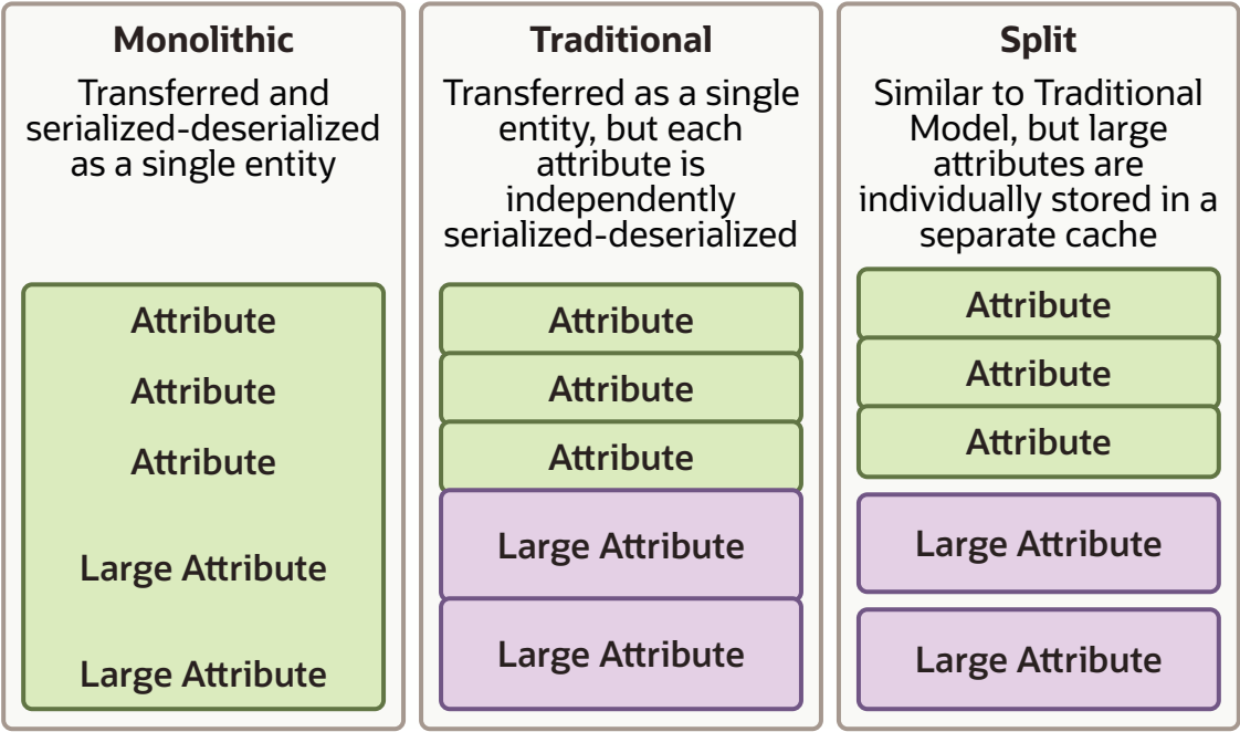
Figure 5-1 Traditional, Monolithic, and Split Session Models
