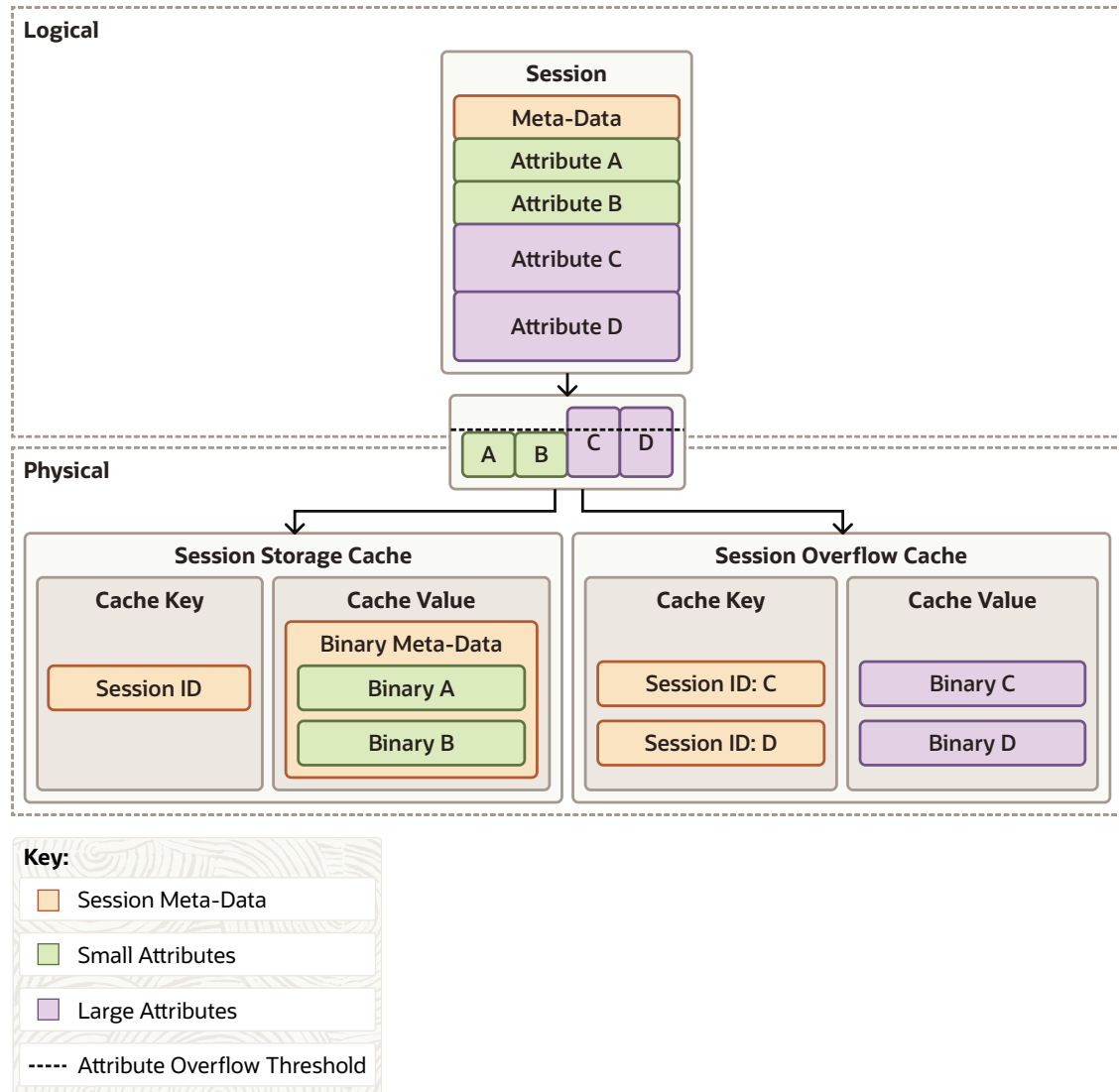
Figure 5-4 Split Session Model
