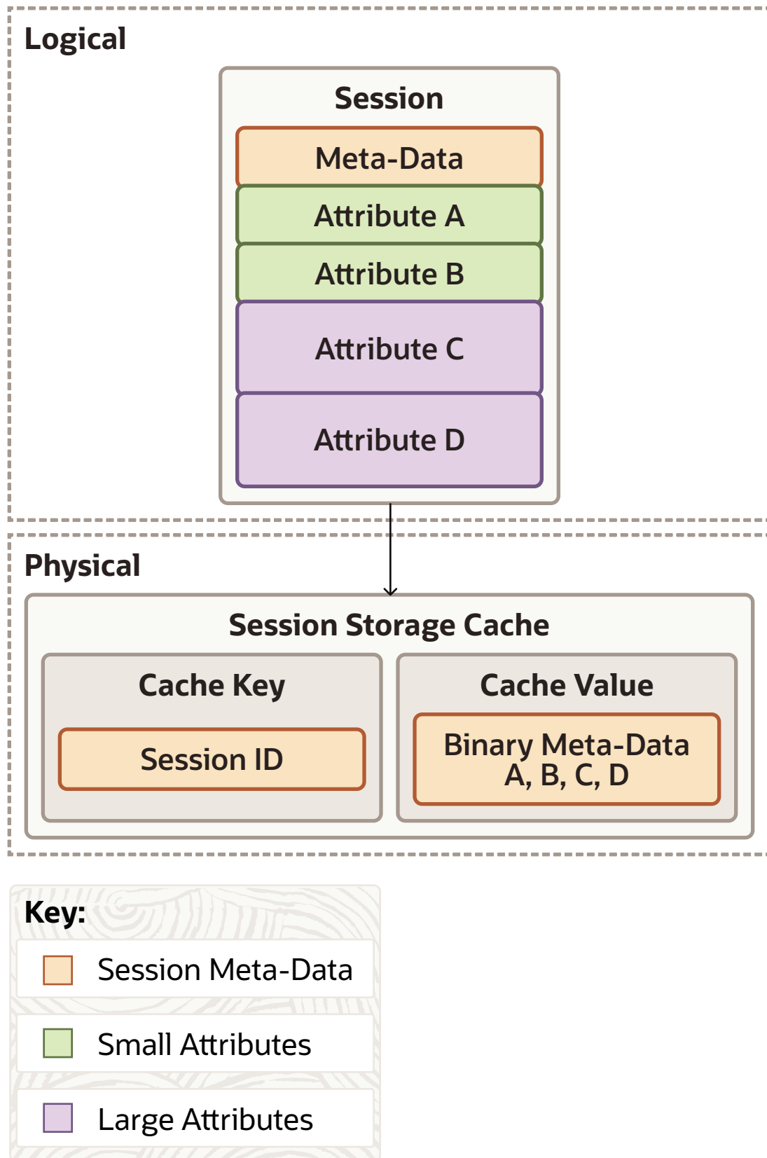
Figure 5-2 Monolithic Session Model
