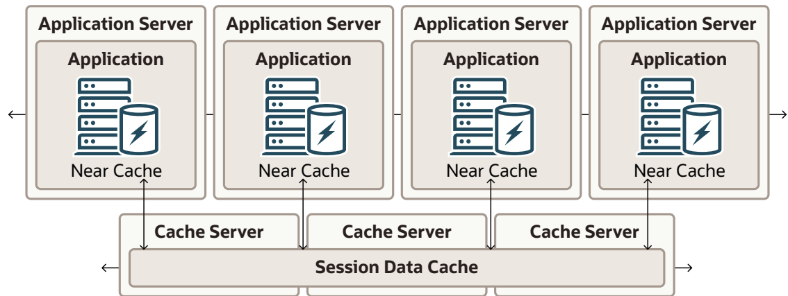
Figure 5-10 Out-of-Process Deployment Topology
