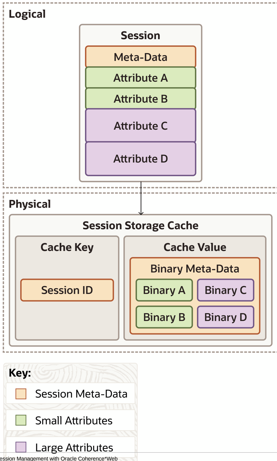
Figure 5-3 Traditional Session Model
