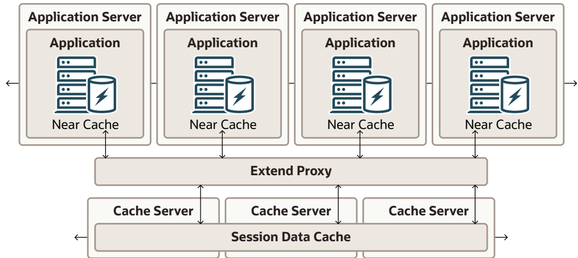
Figure 5-11 Out-of-Process with Coherence*Extend Deployment Topology
