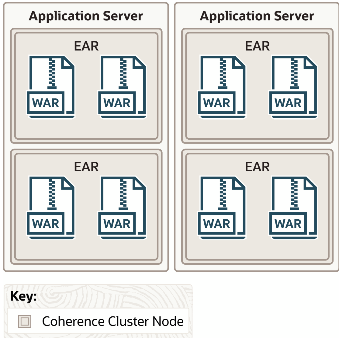
Figure 5-7 EAR-Scoped Cluster
