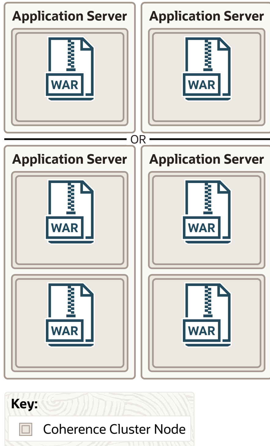
Figure 5-8 WAR-Scoped Clusters
