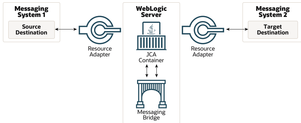
Figure 1-1 WebLogic Messaging Bridge
