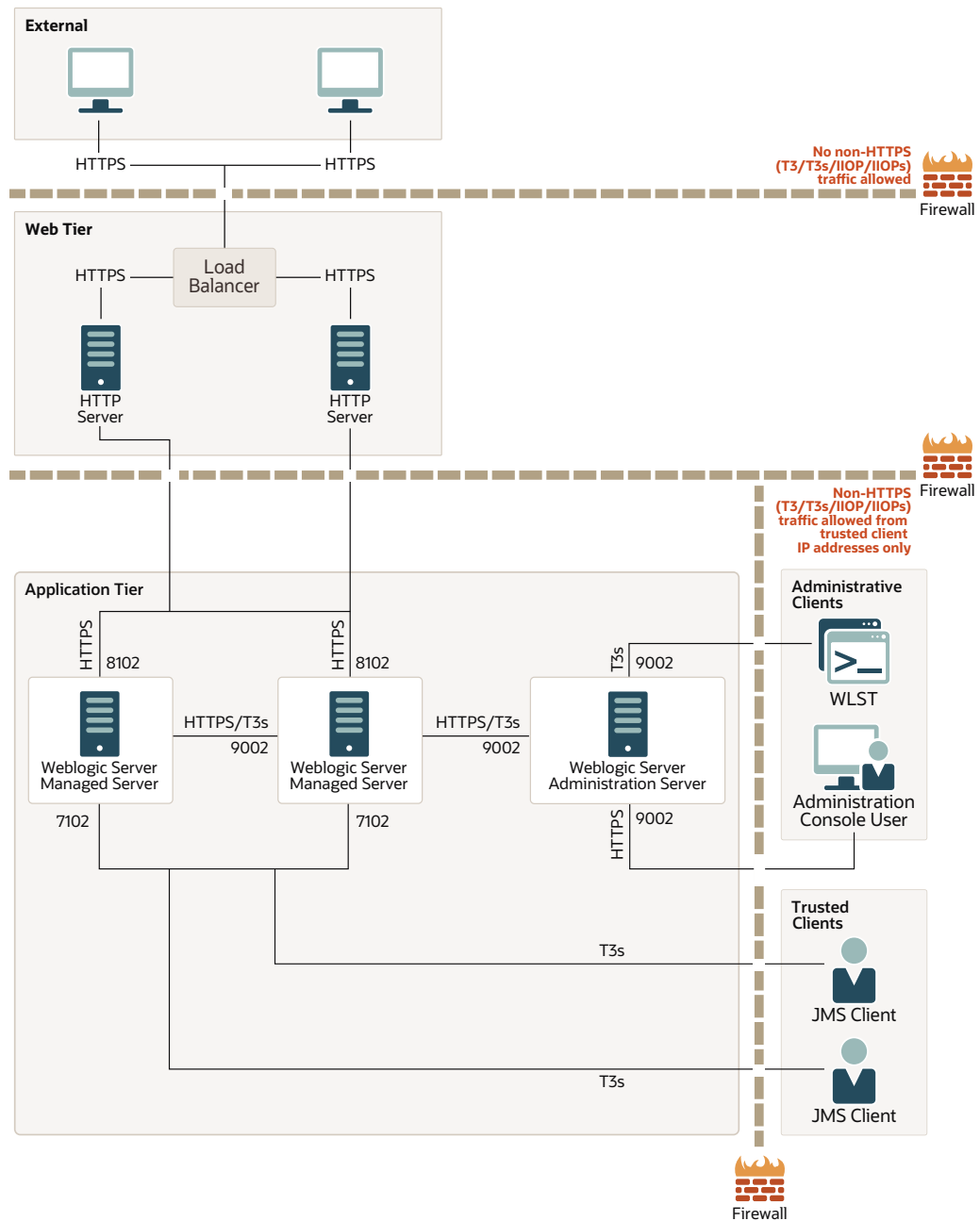
Figure 3-2 WebLogic Server Secure Configuration
