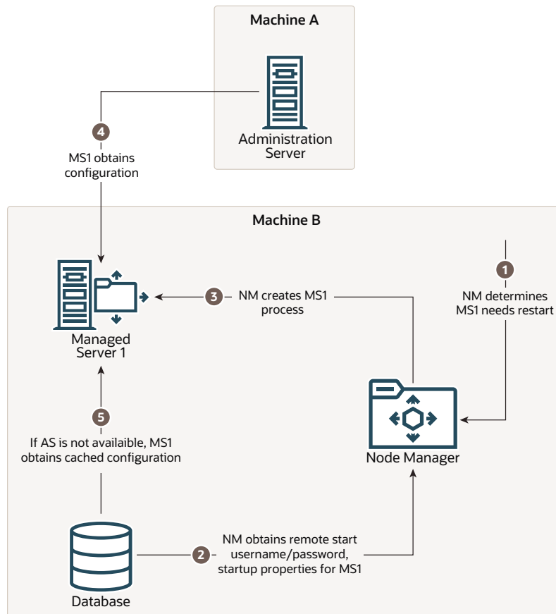
Figure 2-5 Restarting a Managed Server
