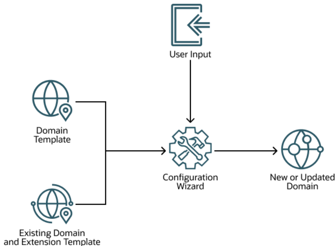
Figure 1-2 Configuration Wizard
