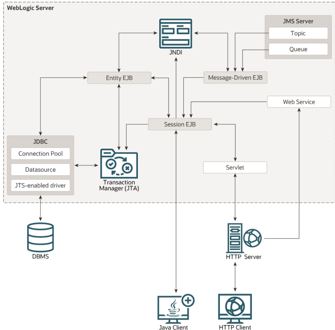
Figure 1-1 EJBs and Other Application Components
