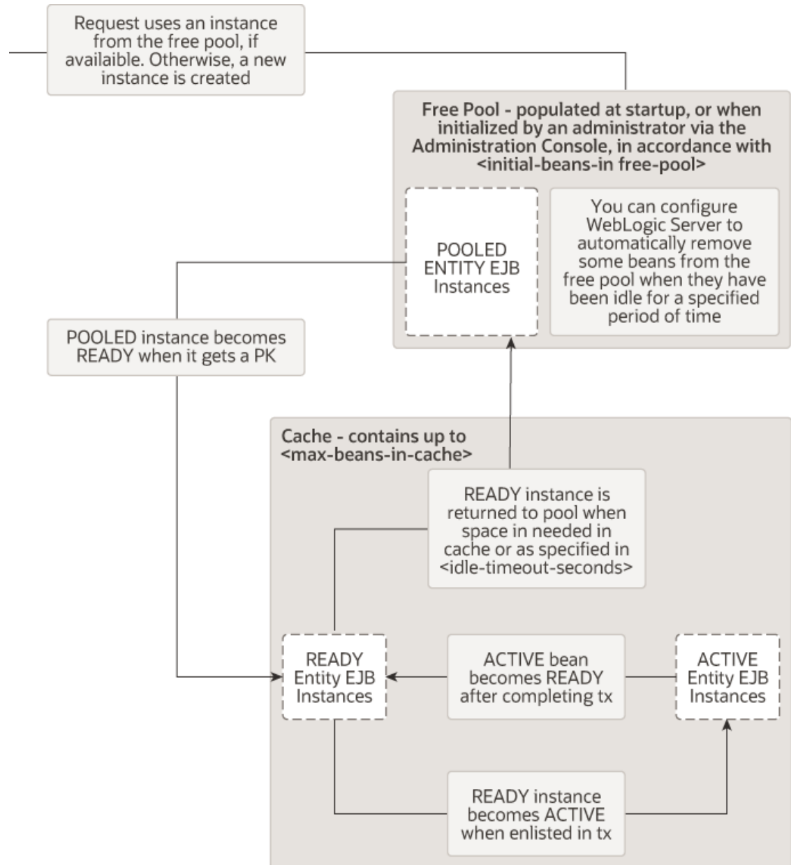
Figure 5-1 Entity Bean Life Cycle
