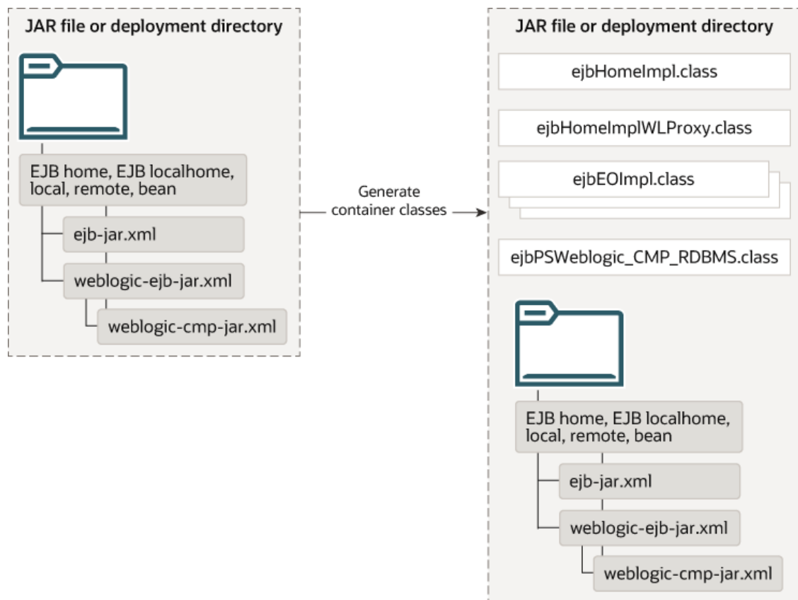
Figure 3-2 Generating EJB Container Classes
