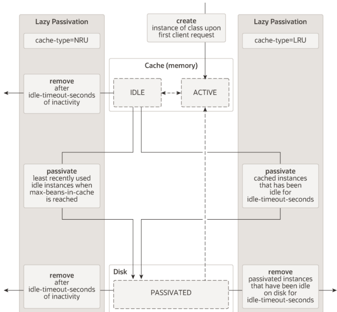
Figure 4-2 Stateful Session EJB Life Cycle
