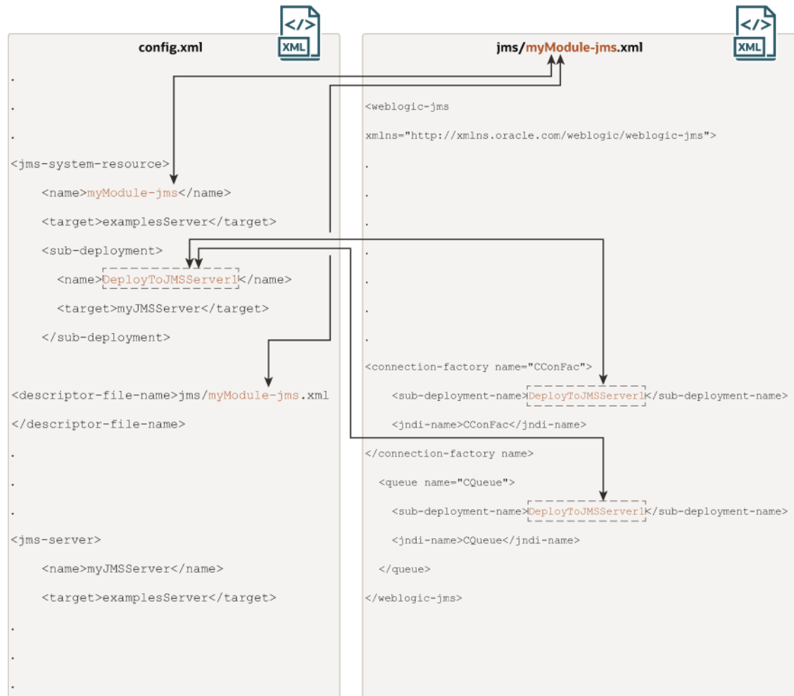
Figure 6-1 Subdeployment Architecture
