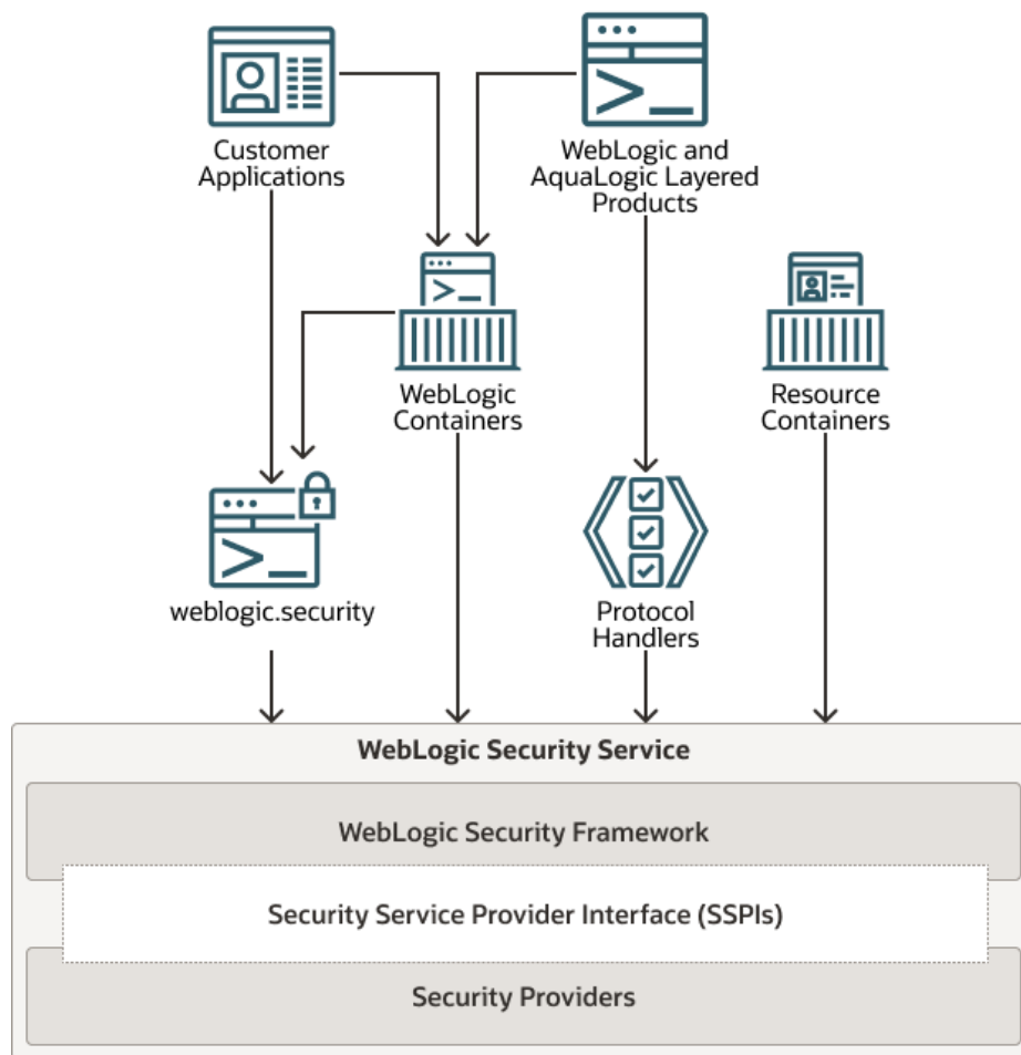
Figure 5-1 WebLogic Security Service Architecture
