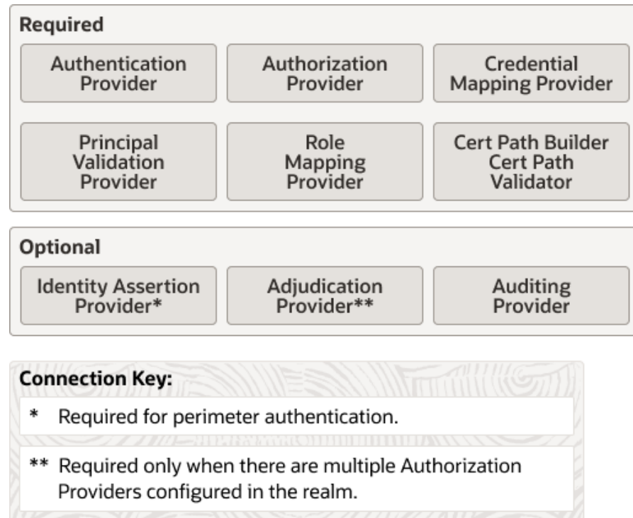
Figure 5-11 WebLogic Security Providers
