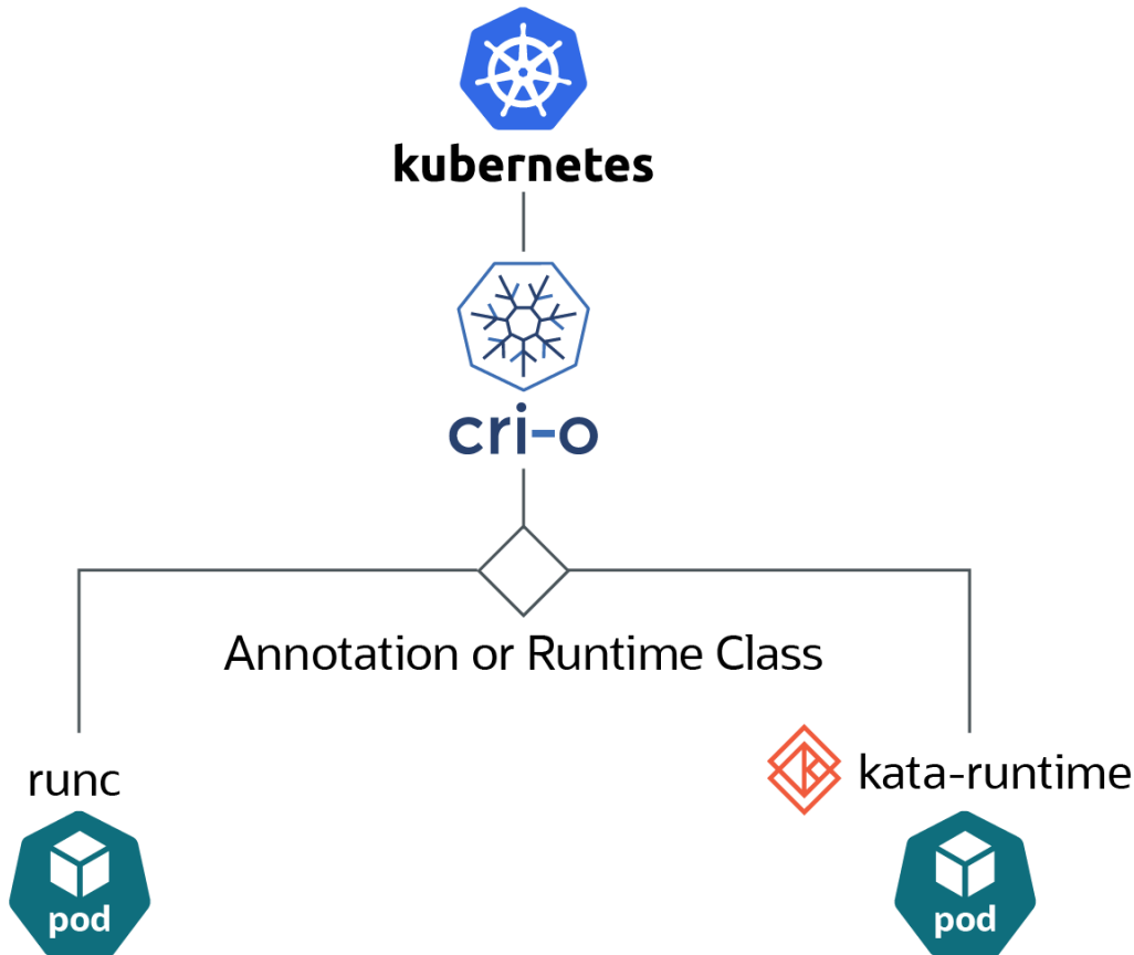
Figure 1.1 Kubernetes Runtimes
