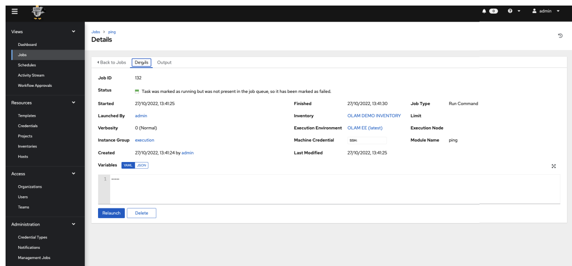
Figure 6-1 Incorrect Status
