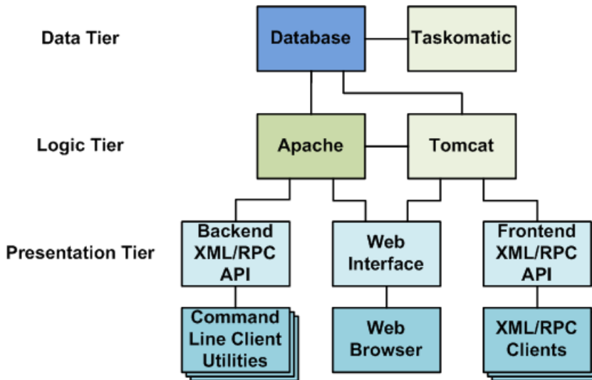
Figure 3.1 Overview of the Internal Three-Tiered Spacewalk Server Architecture
