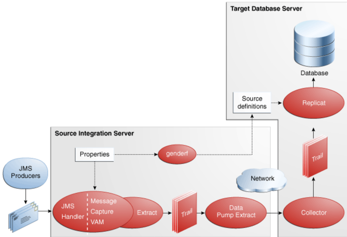
Figure 3–1 Configuration for JMS Message Capture
