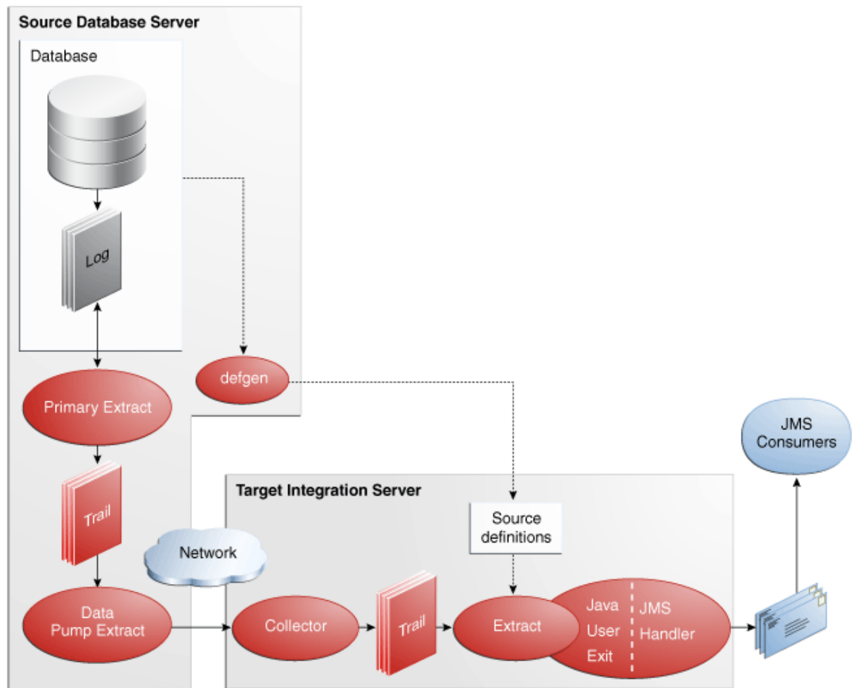
Figure 3–2 Configuration for Delivering JMS Messages
