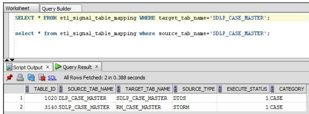
Figure 6 Populating New Columns in the RM Table
