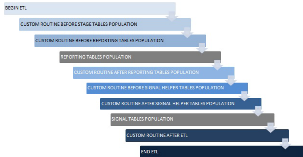
Figure 3 Sequence of ETL Hook Execution
