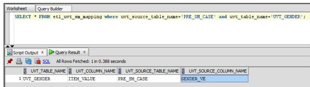
Figure 9 Populating Custom UVT Table
