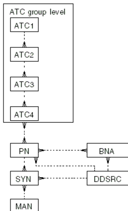
Figure A-6 Sample WHODrug B3 Dictionary Structure
