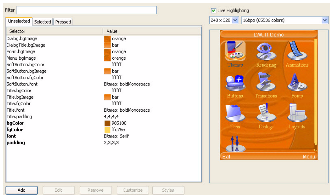
FIGURE 12-6 Theme View When Editing the Default LWUIT Look and Feel
