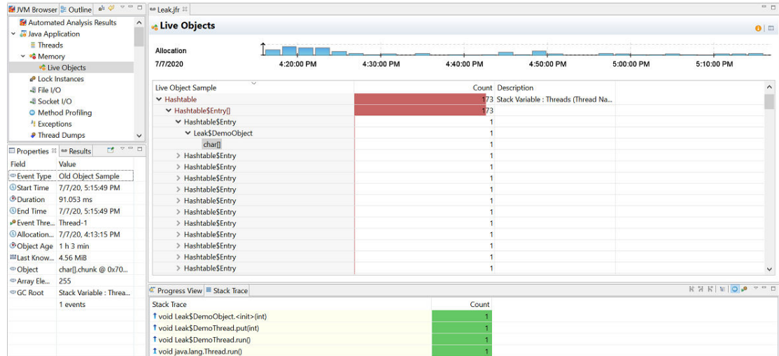
Figure 3-3 Memory Leak - Live Objects Page
