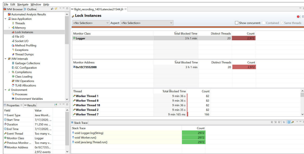
Figure 4-5 Synchronization Issue - Lock Instance
