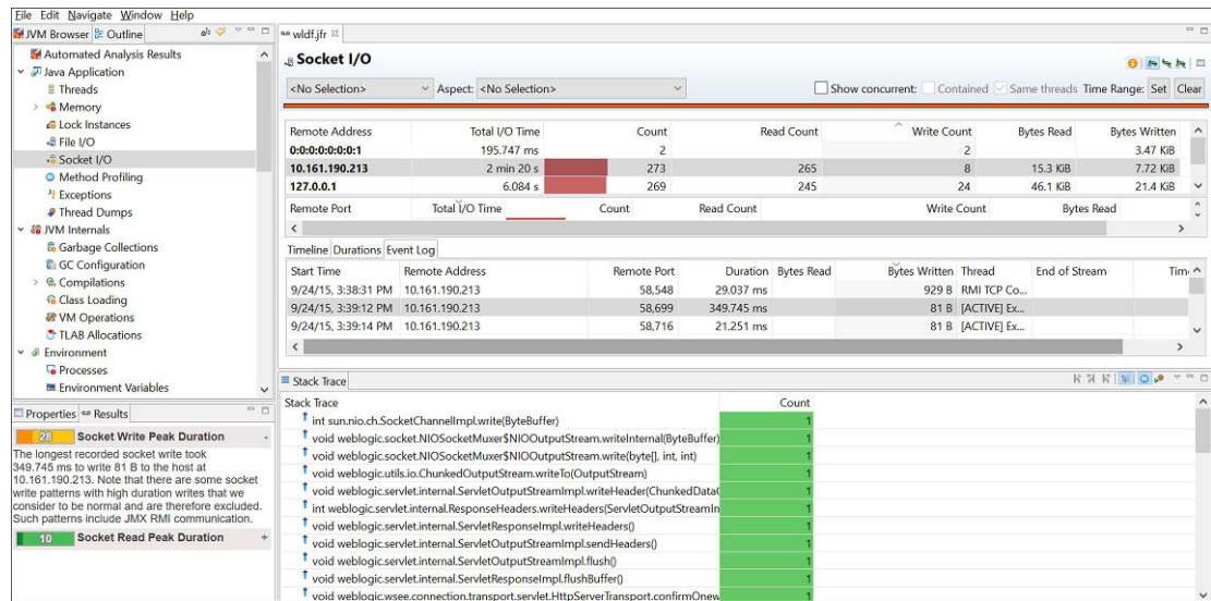
Figure 4-6 Socket I/O - Java Application
