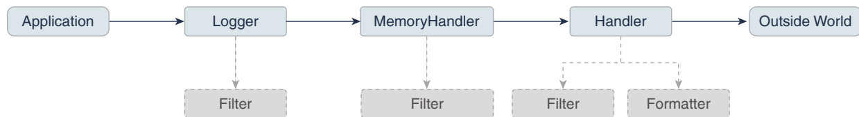
Figure 7-2 Java Logging Control Flow with MemoryHandler
