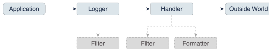
Figure 7-1 Java Logging Control Flow
