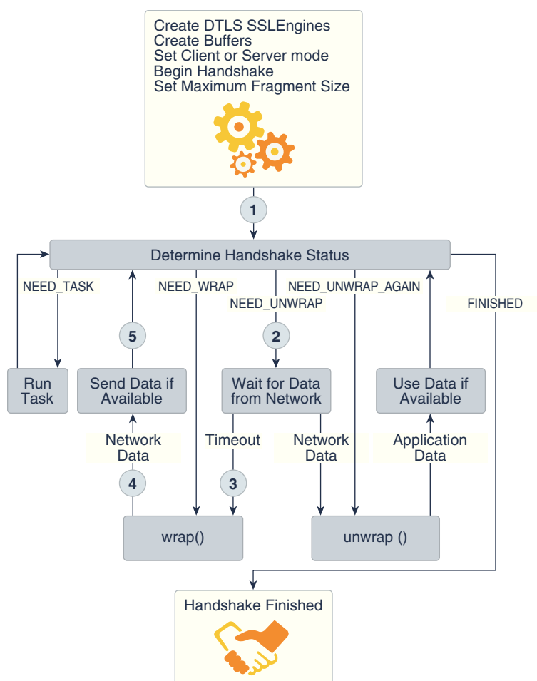
Figure 8-5 DTLS Handshake Retransmission State Flow
