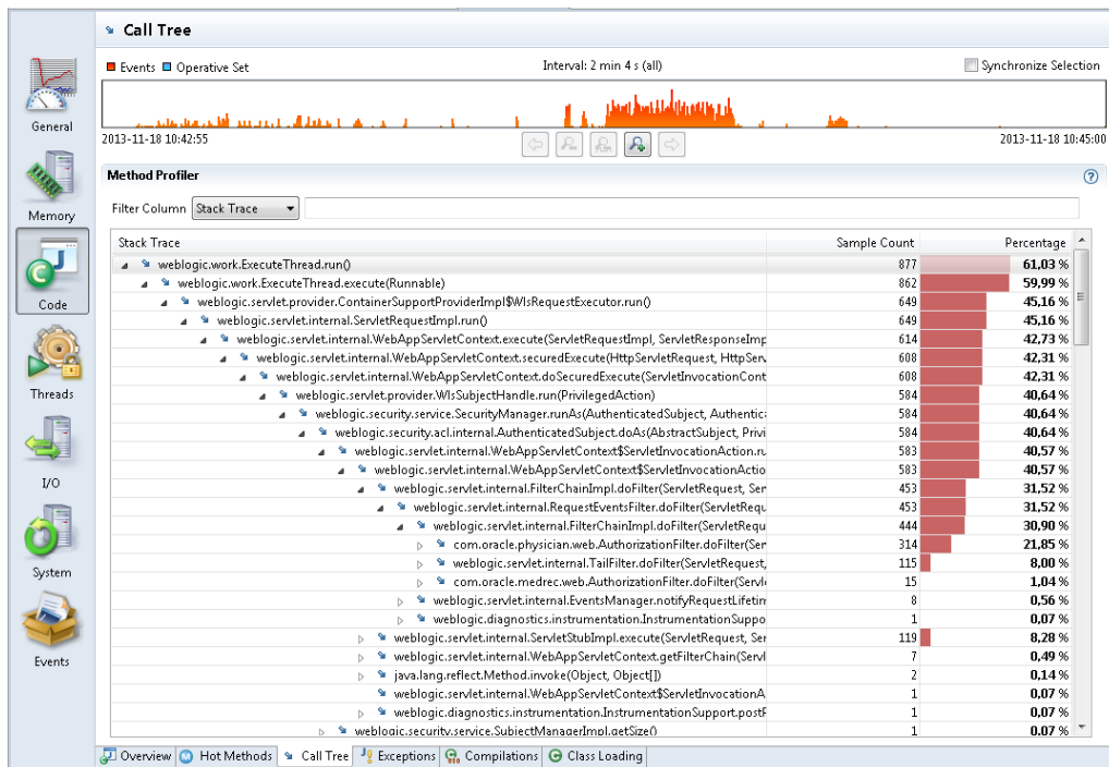
Figure 4-6 Code Execution Performance - Call Tree Tab
