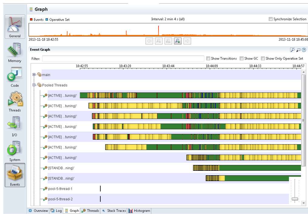
Figure 4-2 Find Bottlenecks - Main Threads from the Graph Tab
