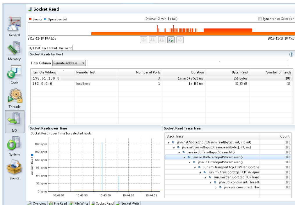
Figure 4-5 I/O Performance Issues - Socket Read Tab
