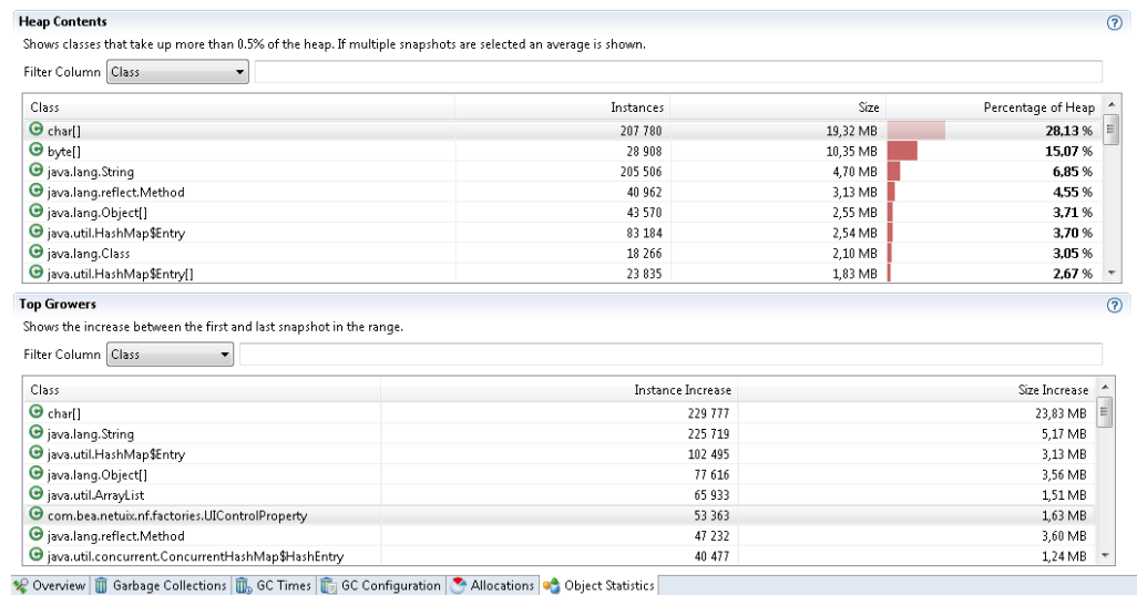
Figure 3-2 Debug Memory Leaks - Find Leaking Class
