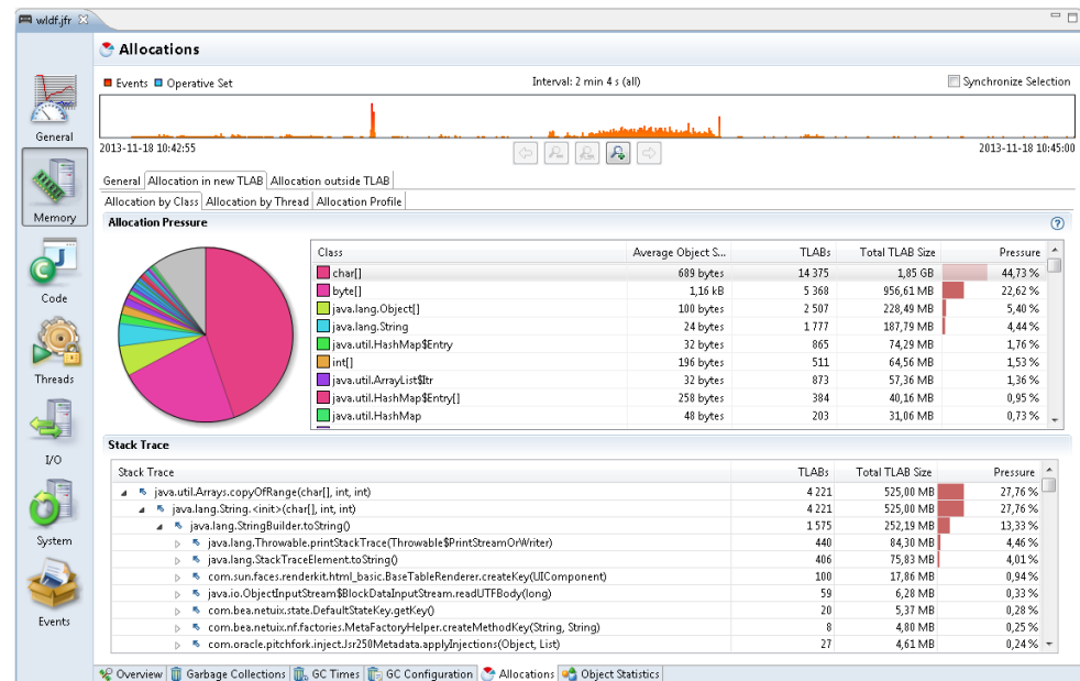
Figure 2-11 Inspect Flight Recordings - Allocations Tab
