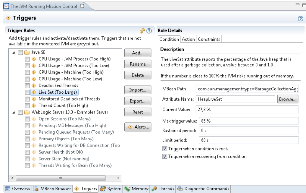
Figure 2-6 Java Mission Control - Automatic Recordings
