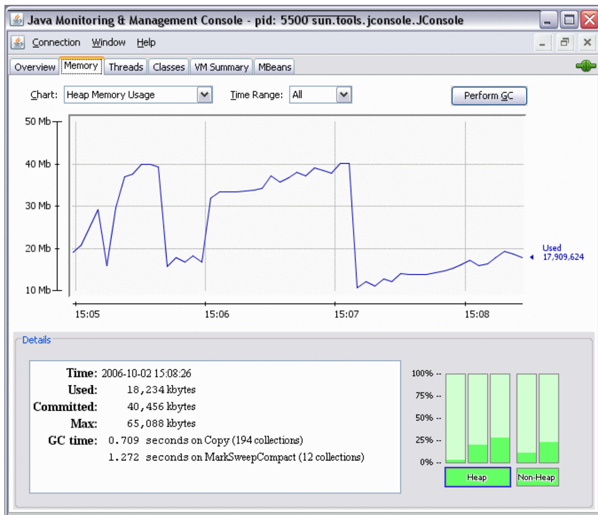
Figure 2-15 Sample Output from JConsole
