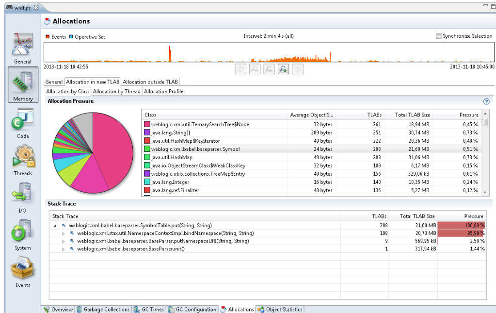
Figure 3-3 Debug Memory Leaks - Allocations tab
