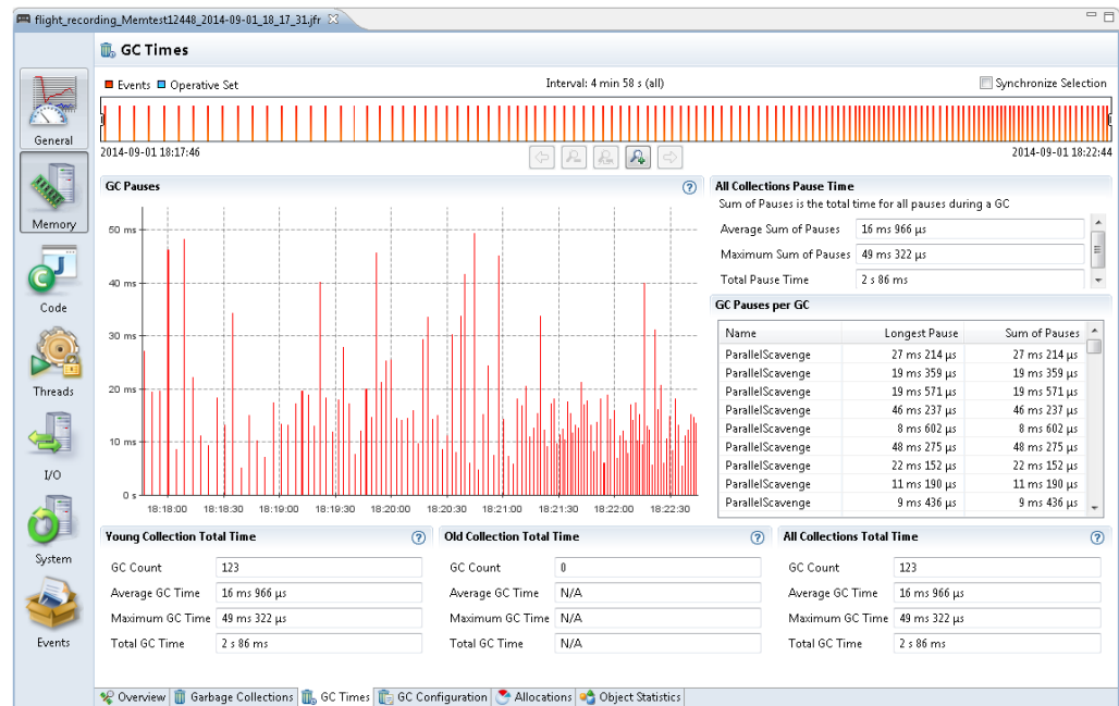
Figure 4-3 Garbage Collection Performance - GC Pauses
