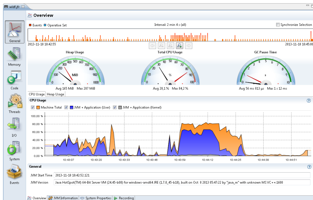
Figure 2-9 Inspect Flight Recordings - General Tab
