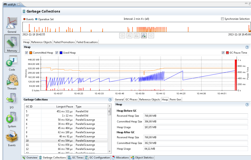
Figure 2-10 Inspect Flight Recordings - Garbage Collections
