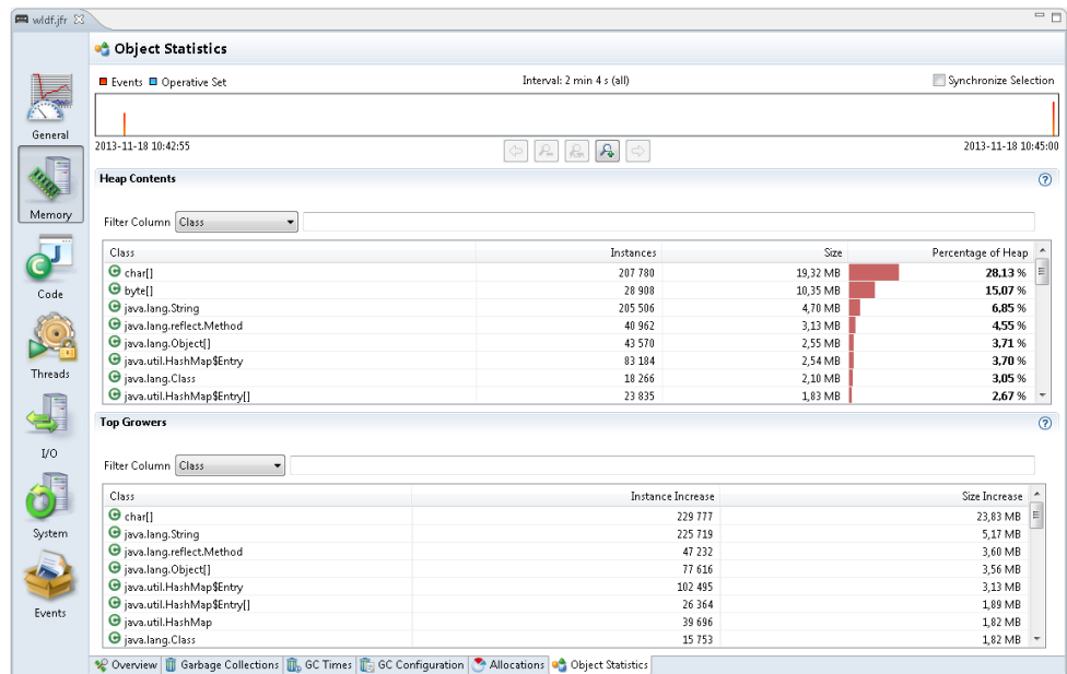
Figure 2-12 Inspect Flight Recordings - Object Statistics Tab
