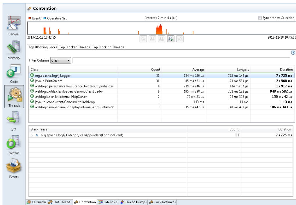
Figure 4-4 Synchronization Performance - Contention Tab
