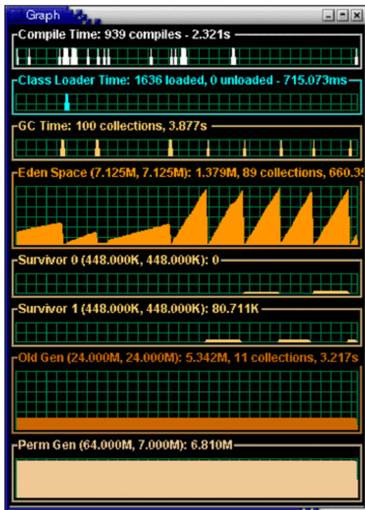
Figure 2-16 Sample Output from visualgc
