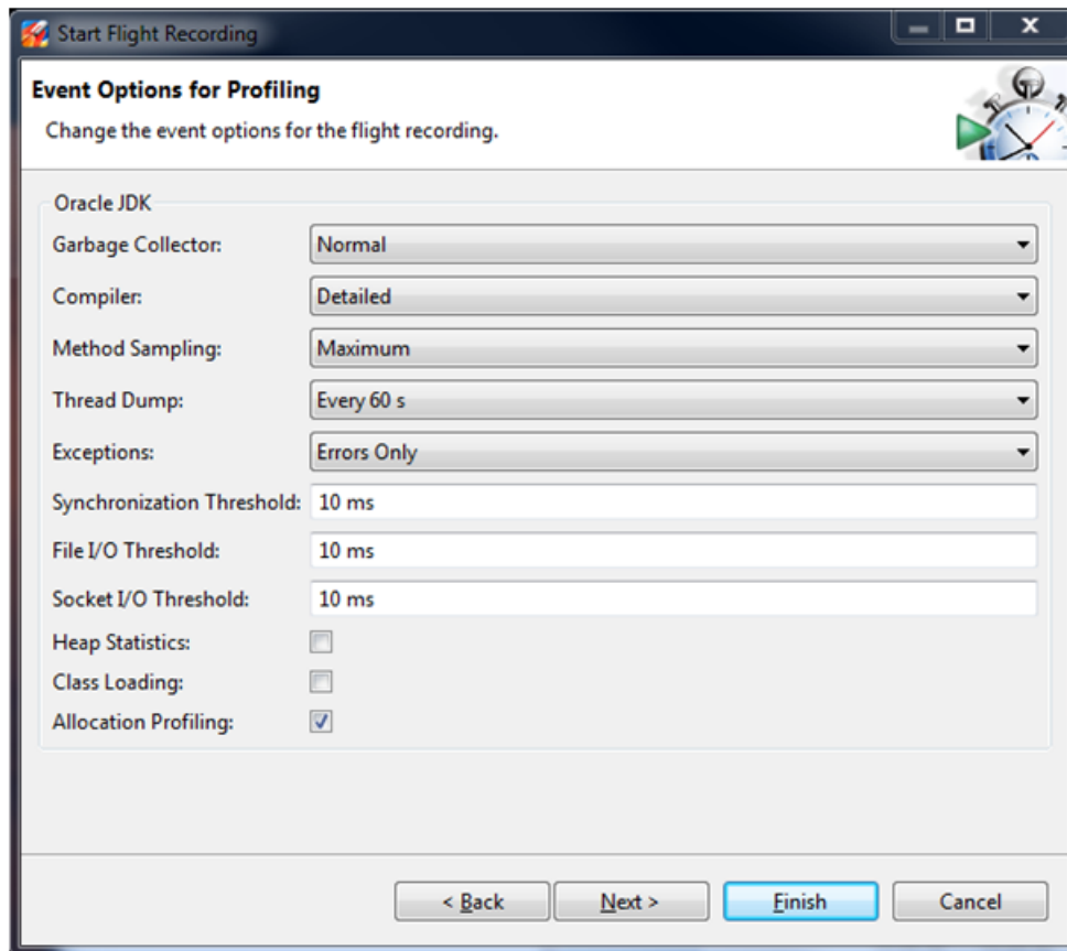
Figure 2-5 Java Mission Control - Event Options for Profiling
