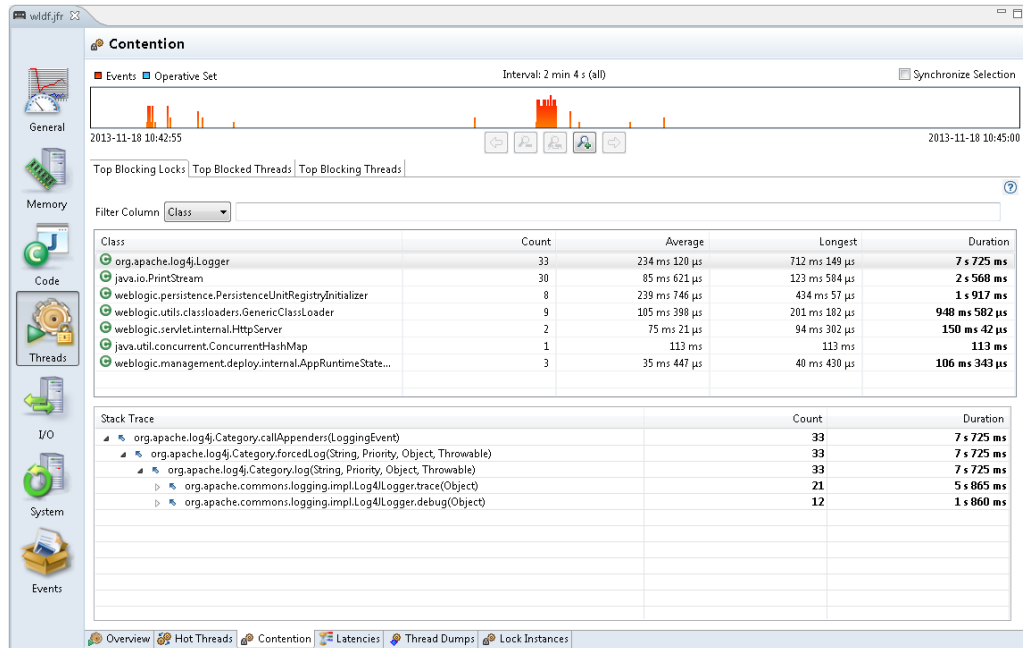
Figure 2-14 Inspect Flight Recordings - Contention Tab
