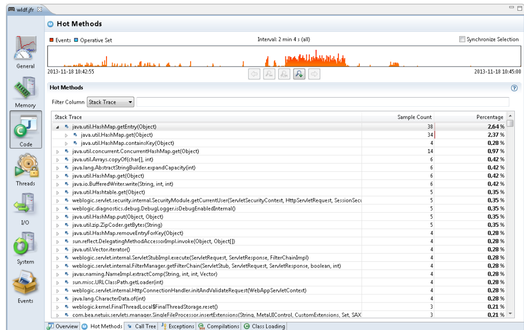
Figure 2-13 Inspect Flight Recordings - Code Tab
