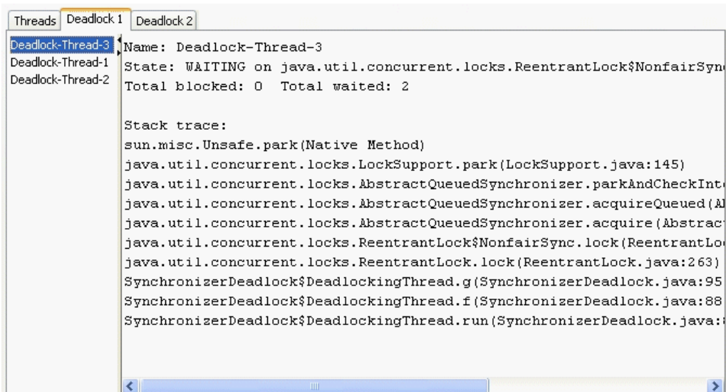
Figure 3-9 Deadlocked Threads
