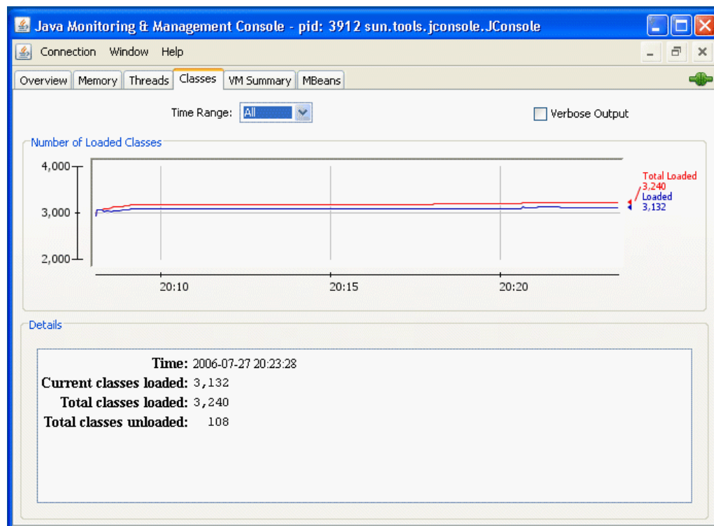
Figure 3-10 Classes Tab
