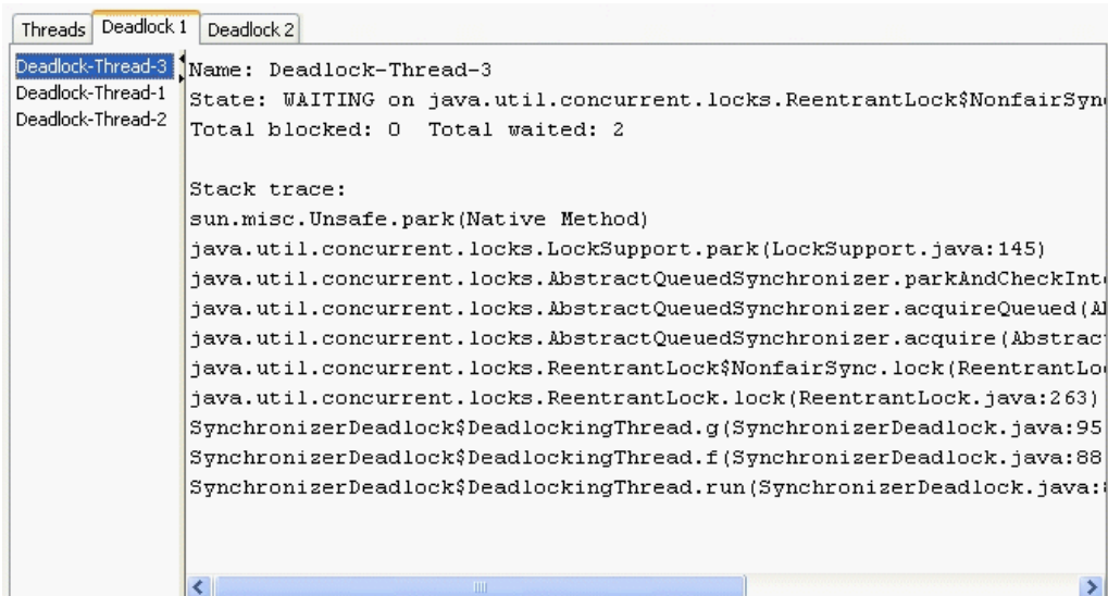
Figure 3-9 Deadlocked Threads
