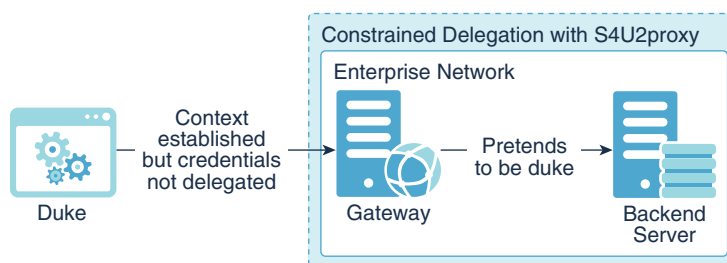
Figure 7-4 Constrained Delegation with S4U2proxy
