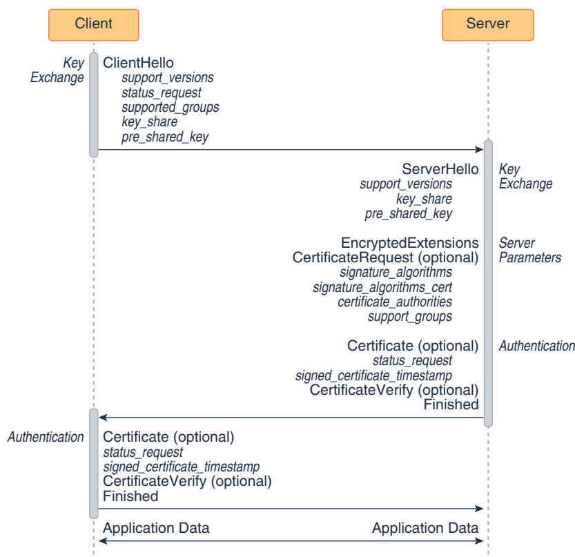
Figure 8-7 TLS 1.3 Handshake
