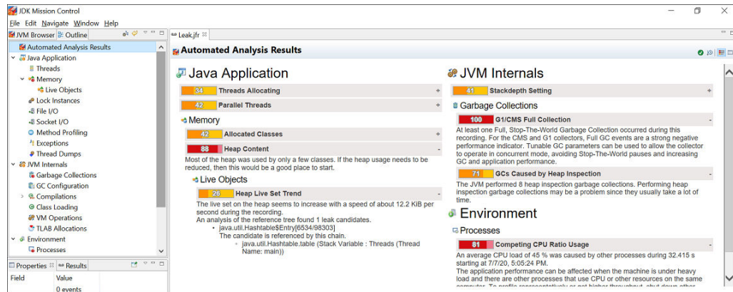
Figure 3-1 Memory Leak - Automated Analysis Page
