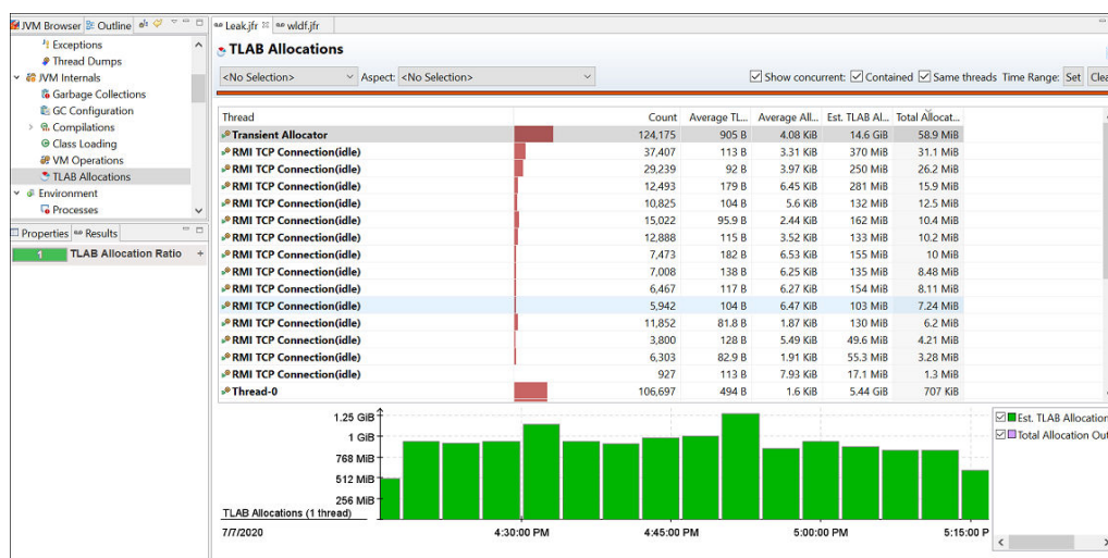
Figure 3-4 Memory Leak - TLAB Allocations
