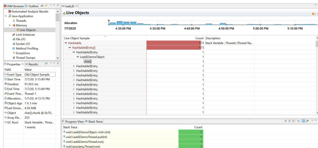
Figure 3-3 Memory Leak - Live Objects Page
