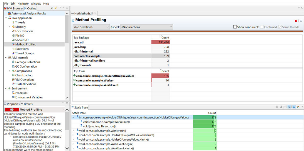
Figure 4-9 Code Execution Performance - Method Profiling
