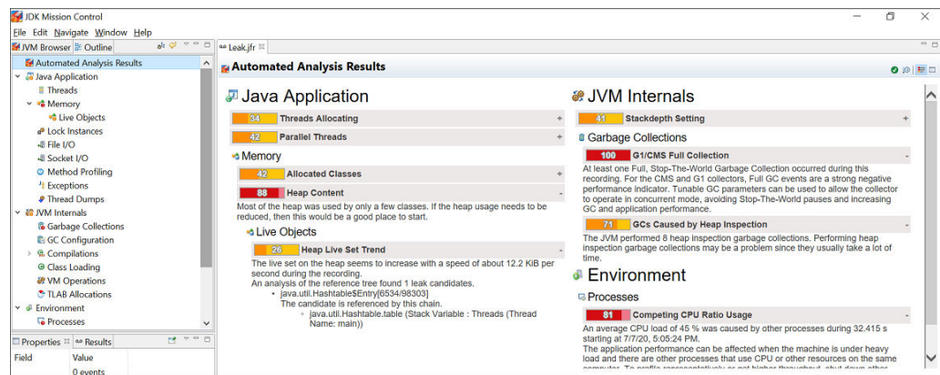
Figure 4-2 Automated Analysis Results - Garbage Collections
