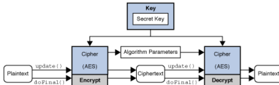
Figure 2-8 The Cipher Class
