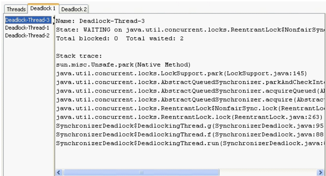
Figure 3-9 Deadlocked Threads
