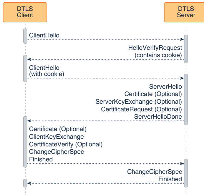
Figure 8-11 DTLS Handshake
